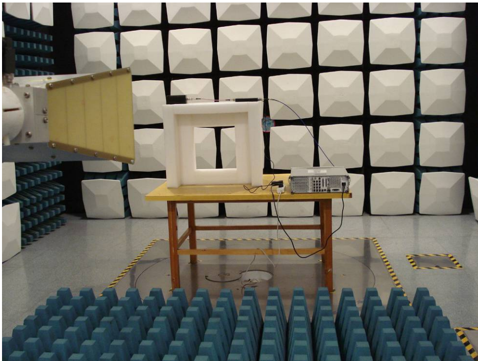
Spurious Emissions Test Setup - Rear View
