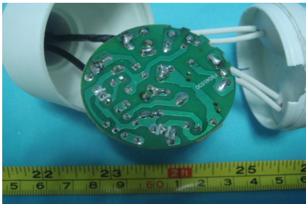
PCB-Back View for ELS-M18
