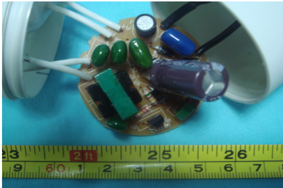
PCB-Back View for ELS-M15
