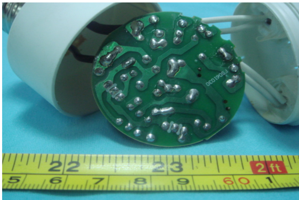
PCB-Back View for ELS-M20
