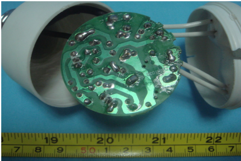
PCB-Back View for ELS-M22
