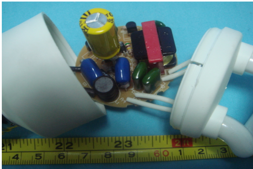
PCB-Front View for ELS-M20
