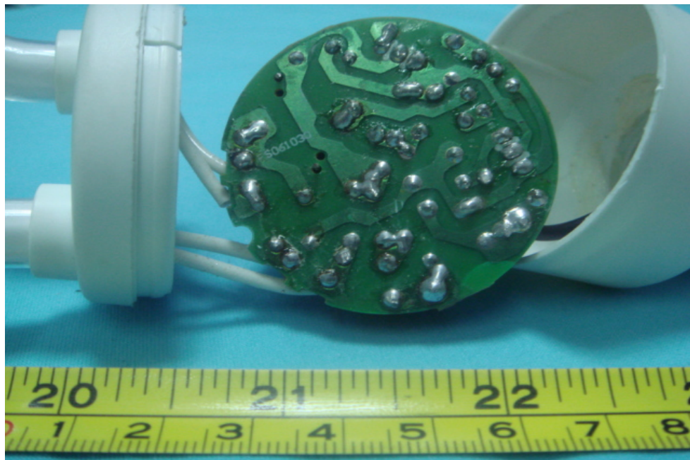
PCB-Back View for ELS-M24(ELS-M23)
