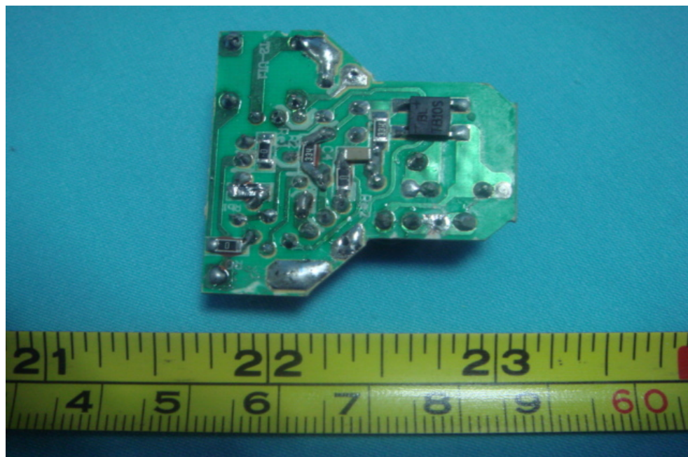
PCB-Back View for ELS-S211
