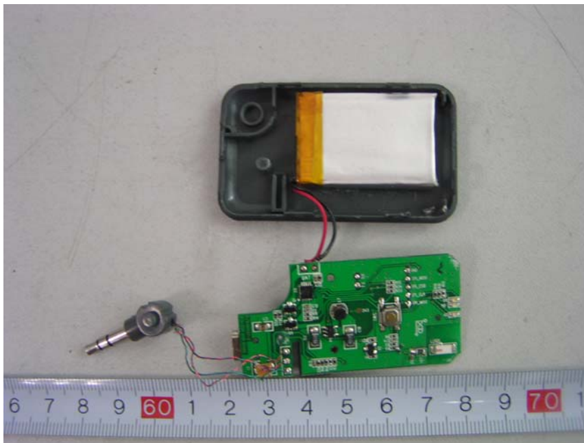
EUT- PCB inside View (2)
