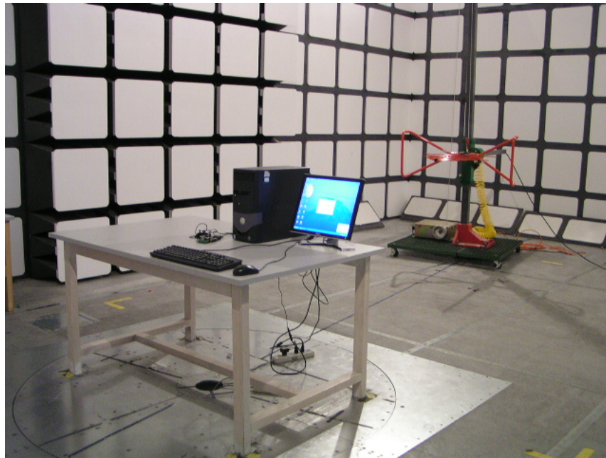
Transmitting Mode: Radiated Emission - Front View (30-1000MHz)
