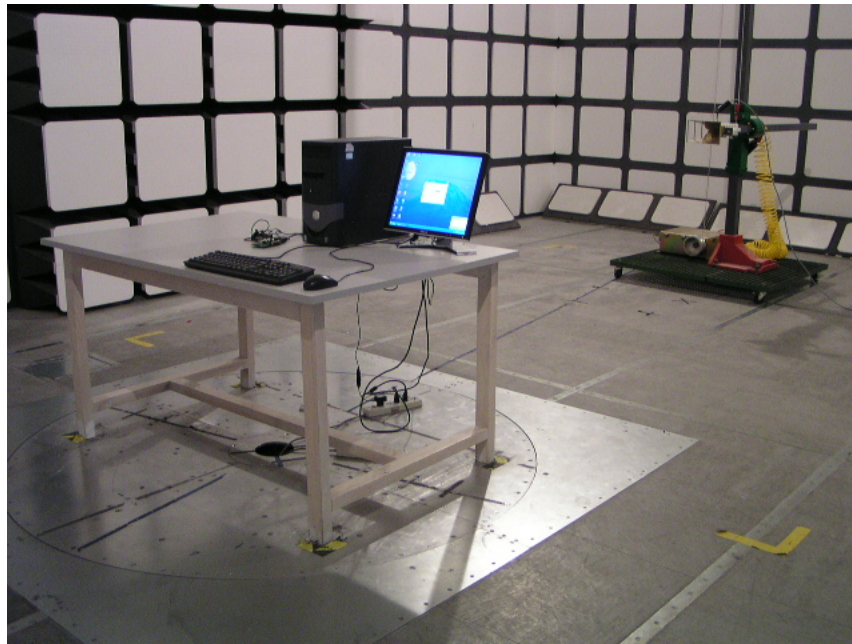
Transmitting Mode: Radiated Emission - Front View (Above 1GHz)
