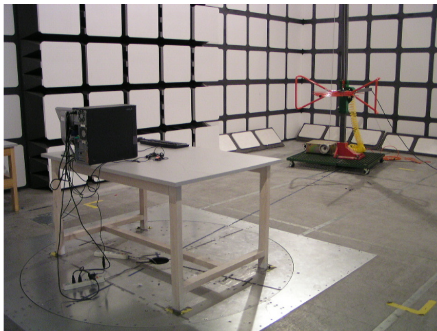
Transmitting Mode: Radiated Emission - Rear View (30-1000MHz)
