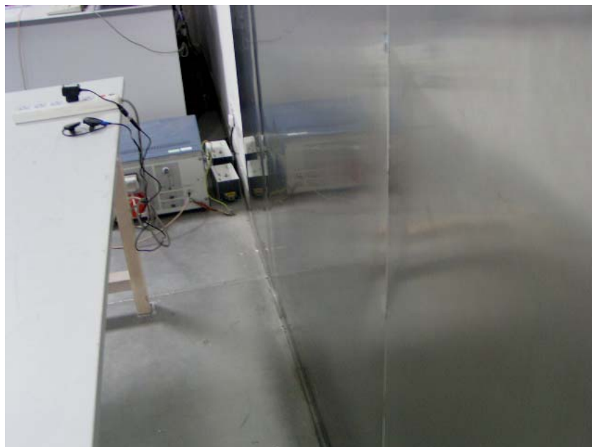
Charging Mode: Conducted Emission - Rear View
