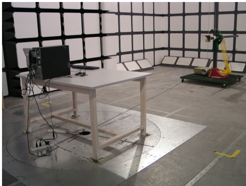
Transmitting Mode: Radiated Emission – Rear View (Above 1GHz)
