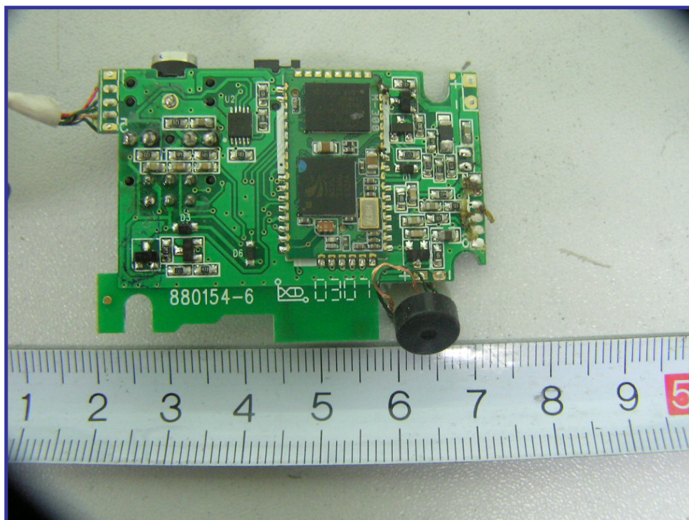
EUT –RF Board Major Component View
