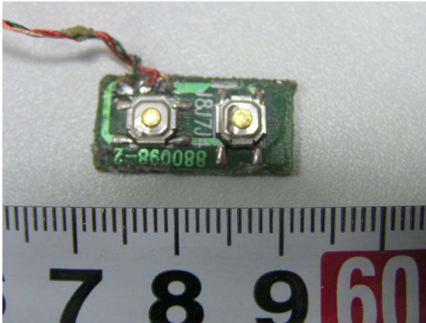
EUT – Key PCB (2) Front View
