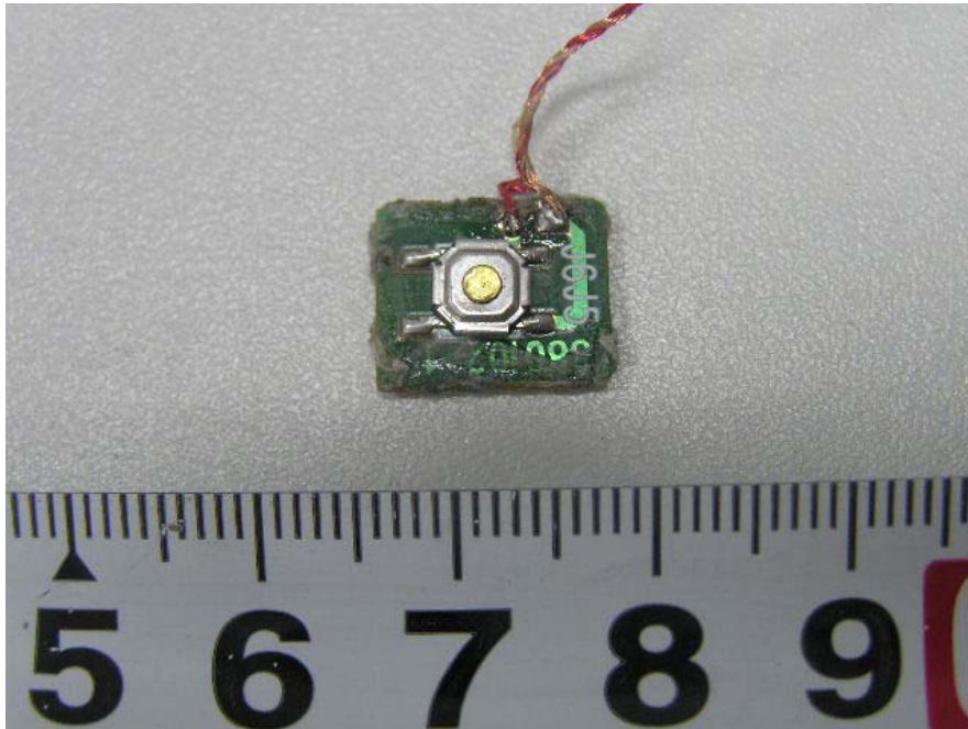
EUT – Key PCB (1) Front View
