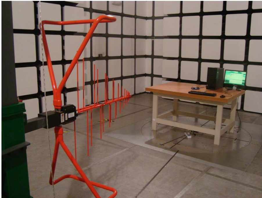
Below 1GHz: Spurious Radiated Emissions - Front View (Transmitting mode)
