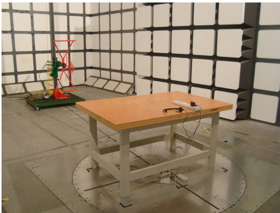
Below 1GHz: Spurious Radiated Emissions - Rear View (Charging by AC adapter)
