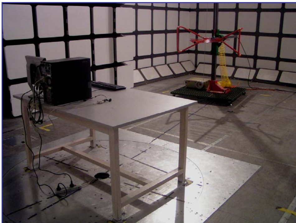
Radiated Emissions - Rear View (30-1000MHz) for transmitting mode
