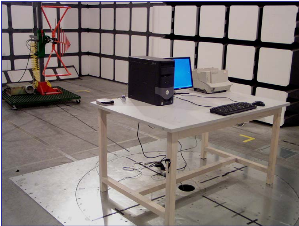
Radiated Emissions - Rear View (Below 1GHz) for charging mode
