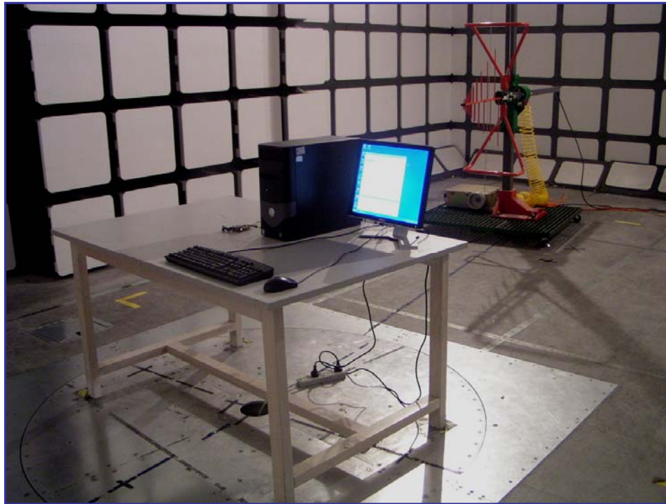
Radiated Emissions - Front View (30-1000MHz) for transmitting mode
