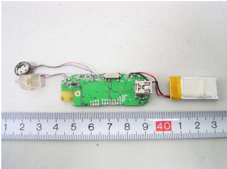
EUT – Mainboard View (3)
