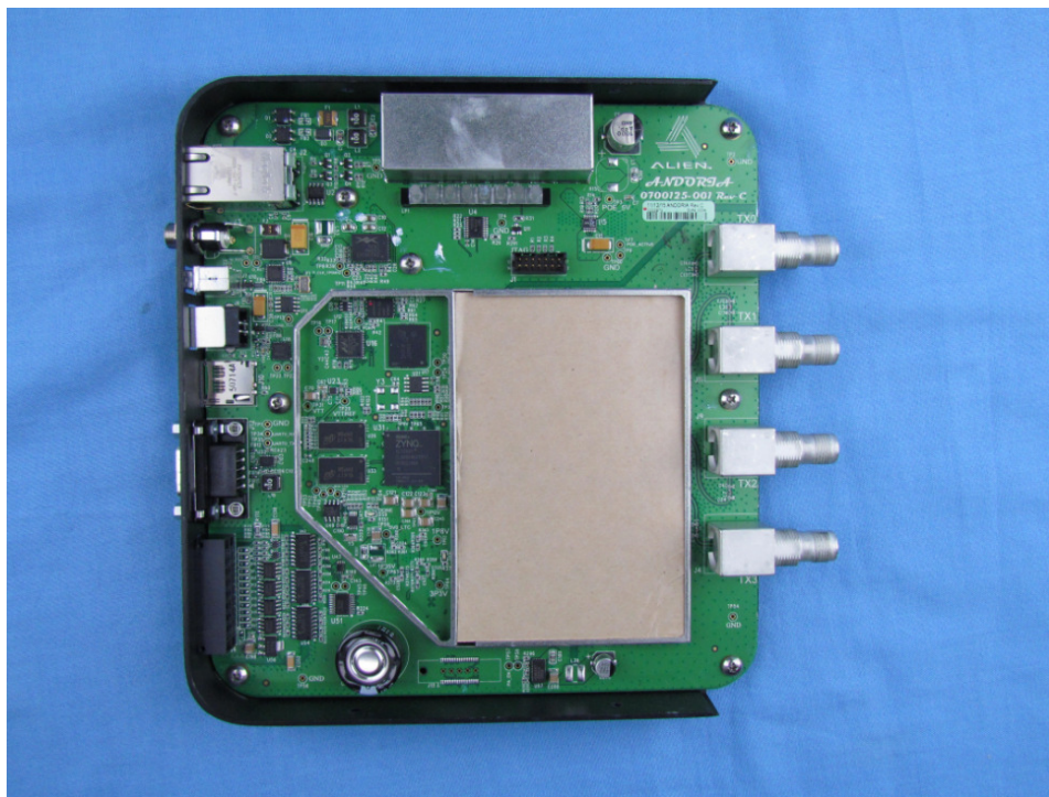
Top View – Shield Off
