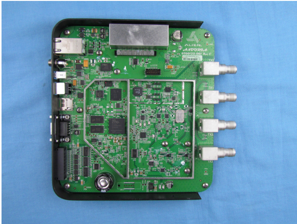
Top View – Shield Off Closer View
