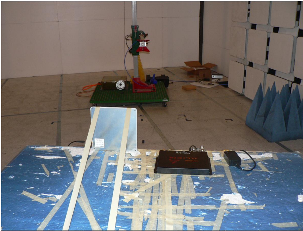
Tx Spurious Emissions 1-18 GHz Antenna 3 Back
