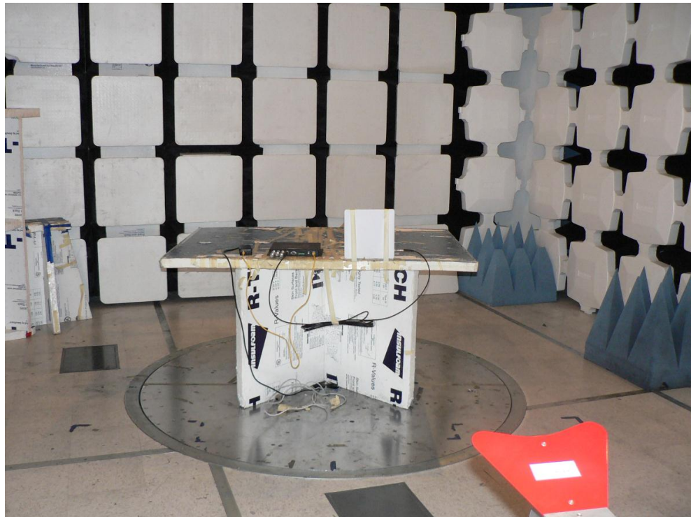
Tx Spurious Emissions 1-18 GHz Front Antenna 1
