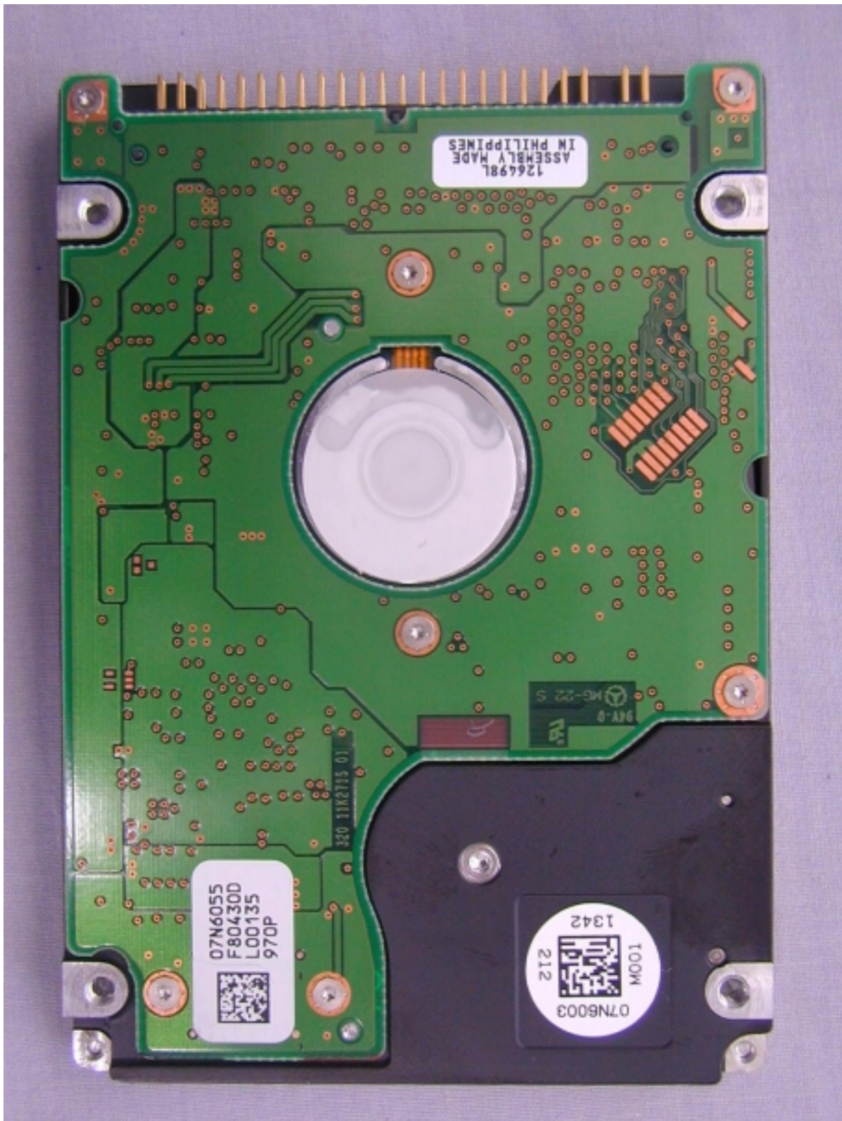
<REAR VIEW OF HDD>
