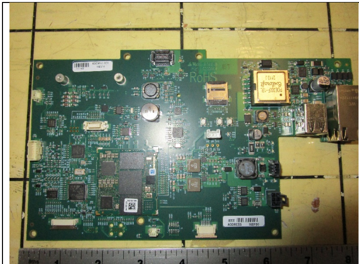
Figure 17: EUT Motherboard - Front
