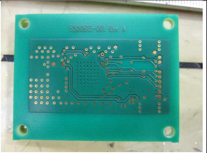
Figure 12: Legic SmartCard Reader - Back
