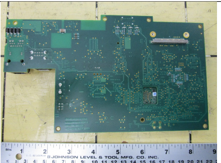
Figure 18: EUT Motherboard - Back
