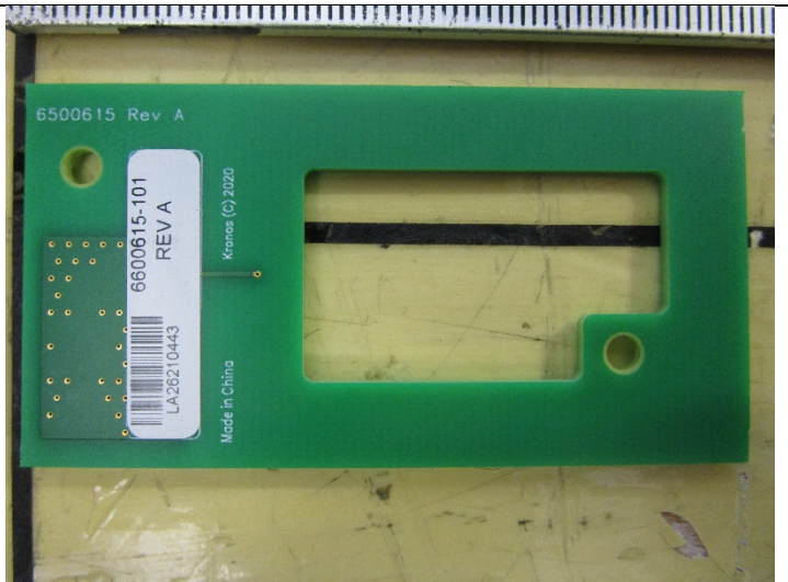
Figure 14: Antenna - Back
