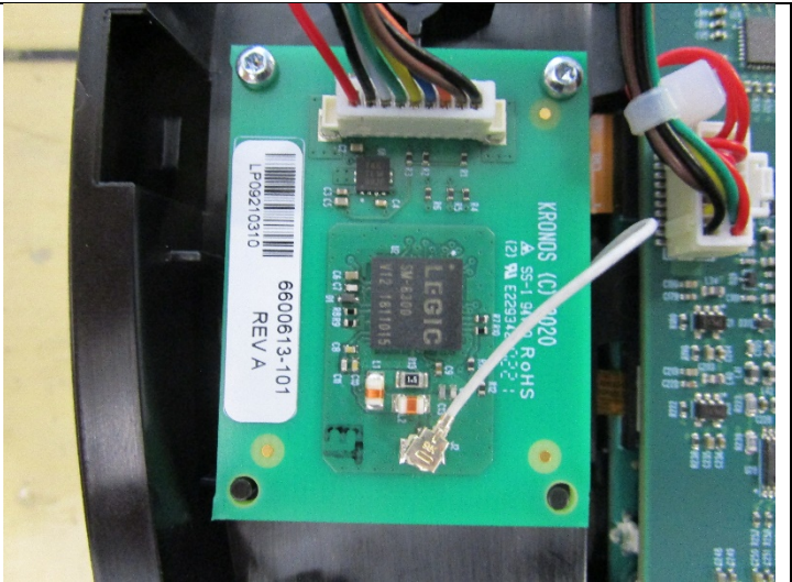
Figure 6: Legic SmartCard Reader
