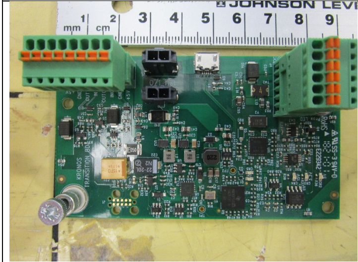
Figure 19: Power Transition Board
