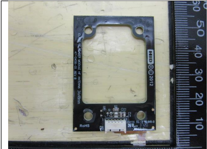
Figure 13: HID Antenna - Front
