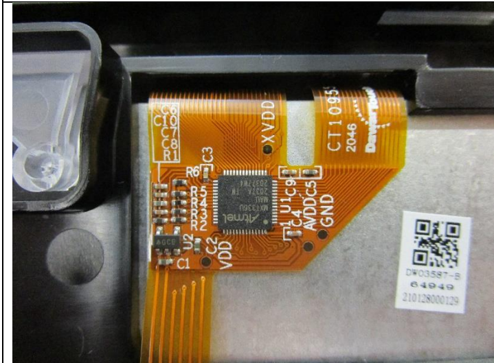
Figure 7: Display Transition Circuit
