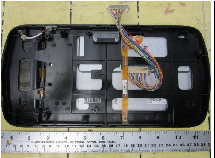
Figure 6: Display Back
