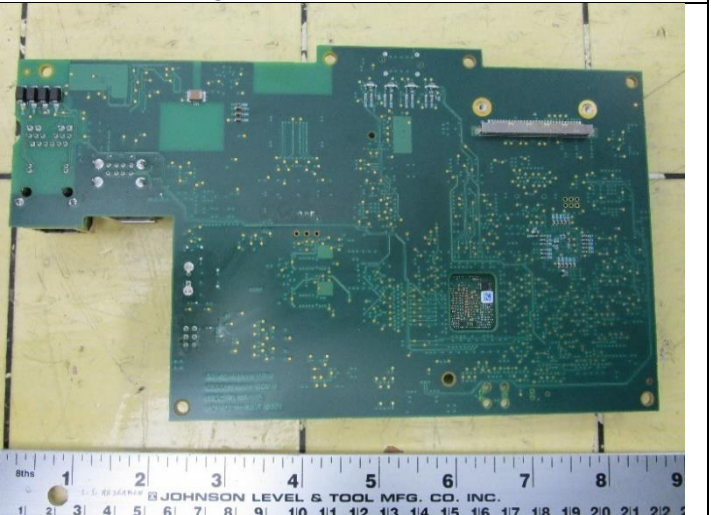
Figure 16: EUT Motherboard - Back
