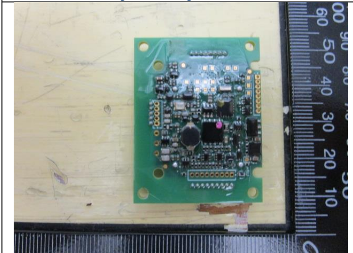
Figure 11: Legic SmartCard Reader - Back
