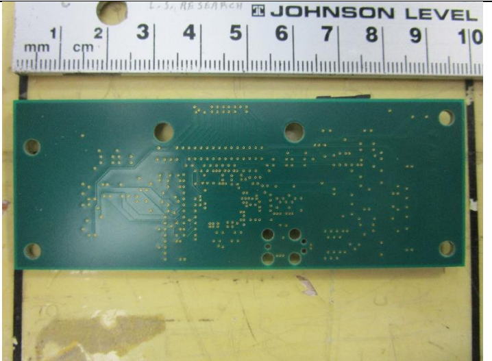
Figure 20: External Input Transition Board - Back
