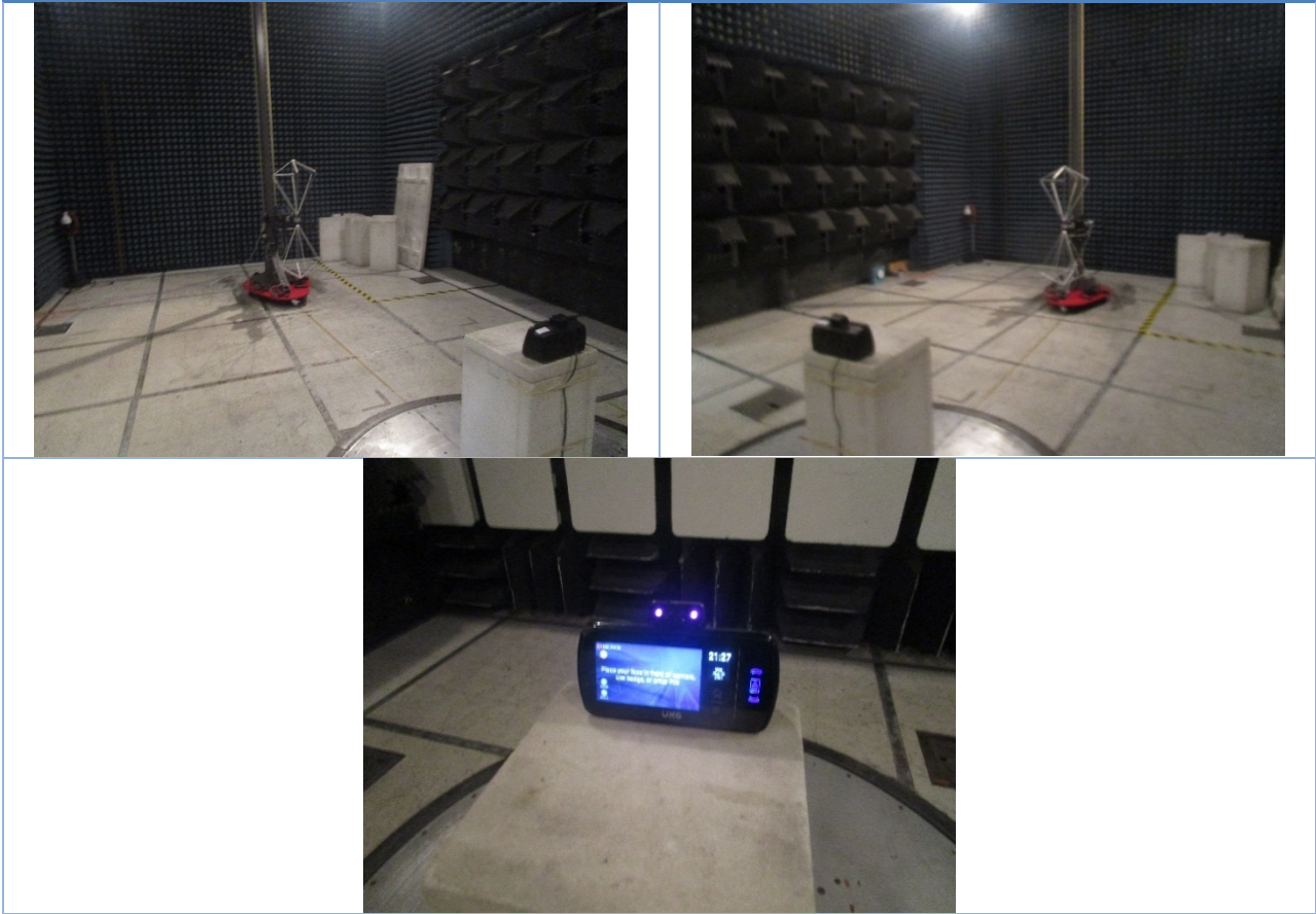
Radiated Emissions: FCC 15.209/RSS-210 | 30-1000 MHz
