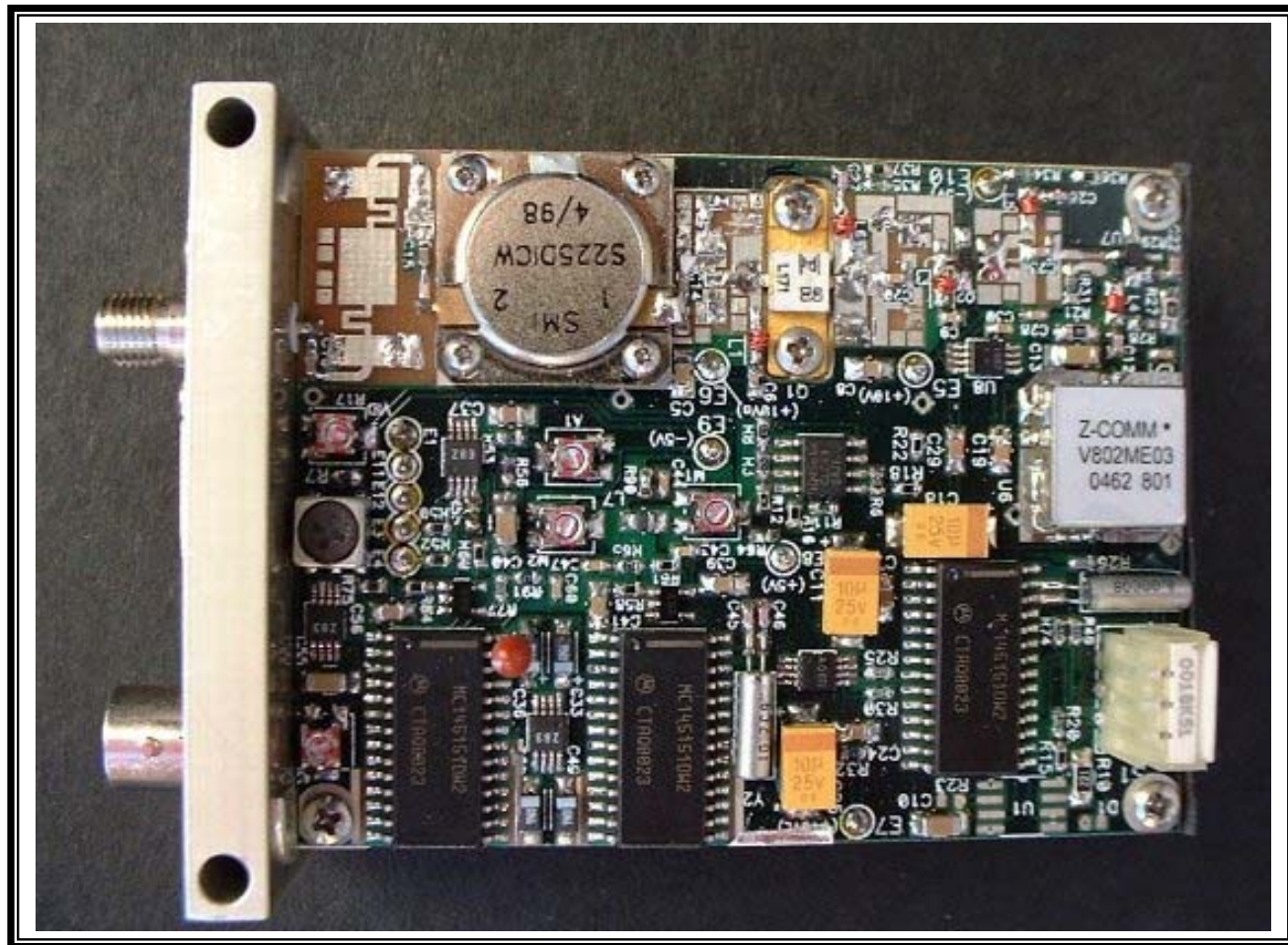
AT-100S RF Board Top Side
