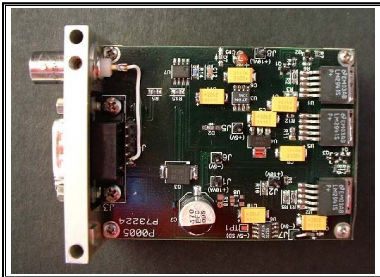
AT-100S Power Supply Top Side
