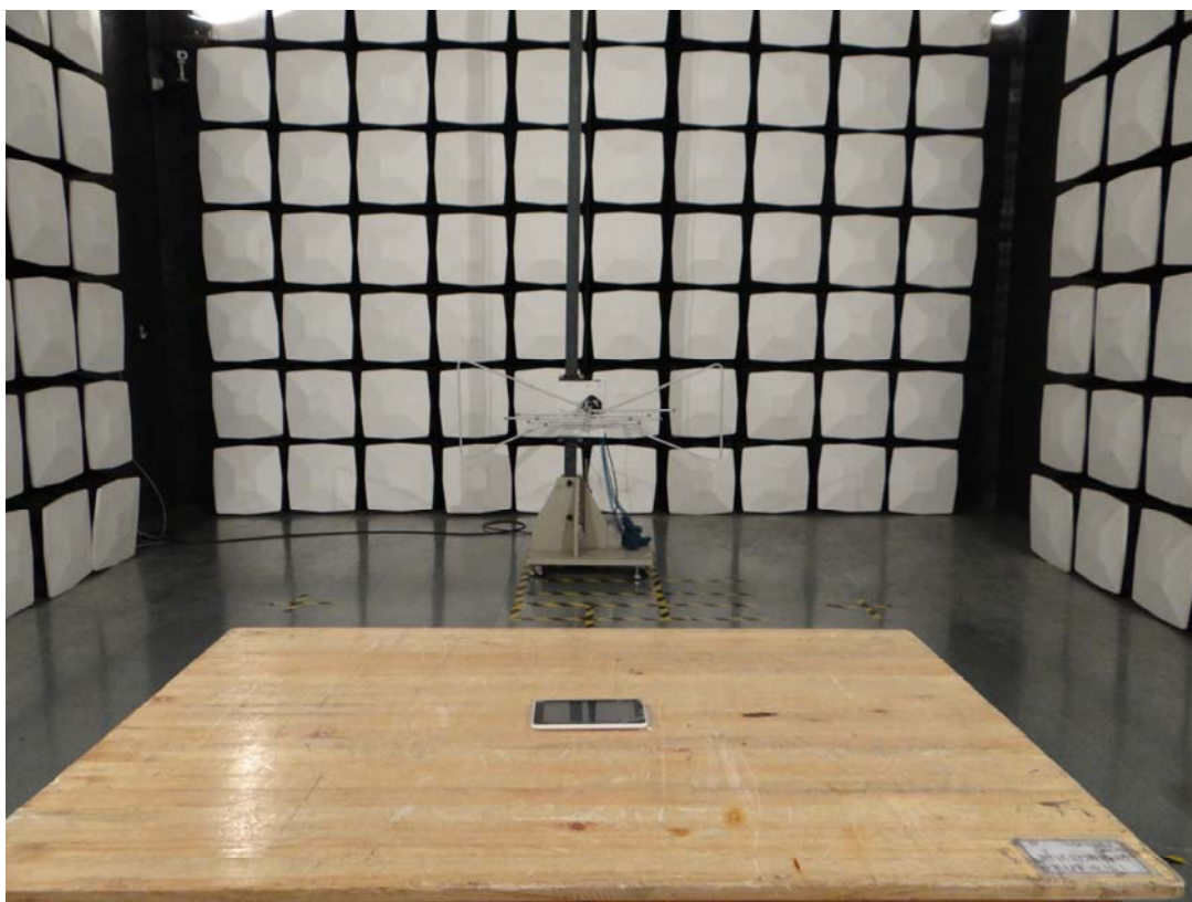
Radiated emission
