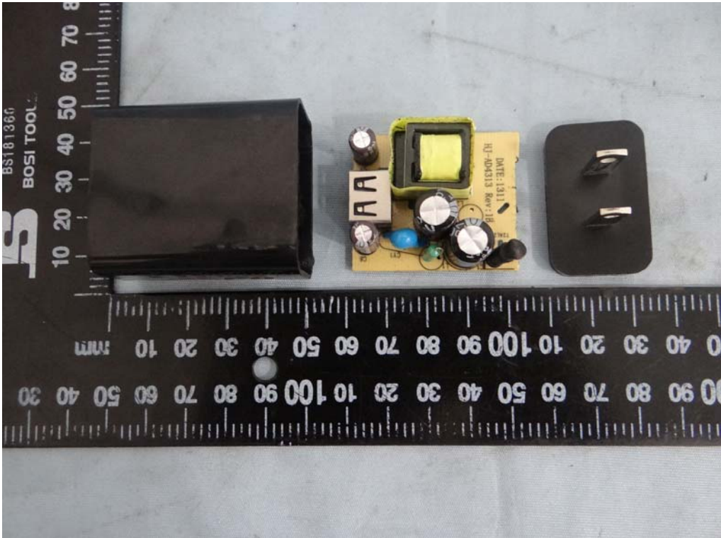
Adapter
