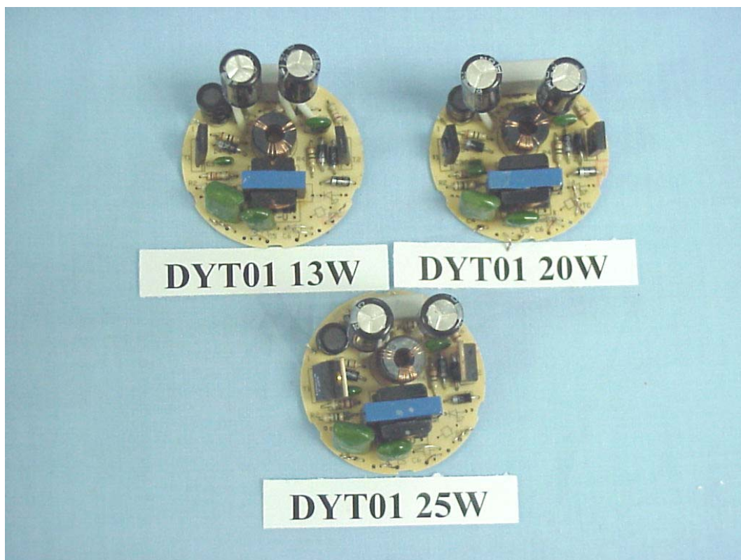
Figure 8 ENERGY SAVING LAMP (M/N: DYT01 13W 20W 25W) MAIN BOARD (COMPONENT SIDE)
