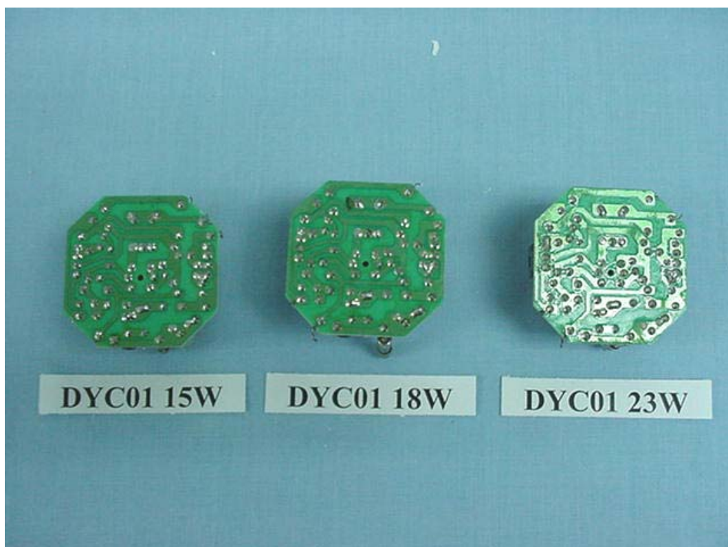
FIGURE 18 ENERGY SAVING LAMP (M/N: DYC01 15W 18W 23W) MAIN BOARD (SOLDERED SIDE)
