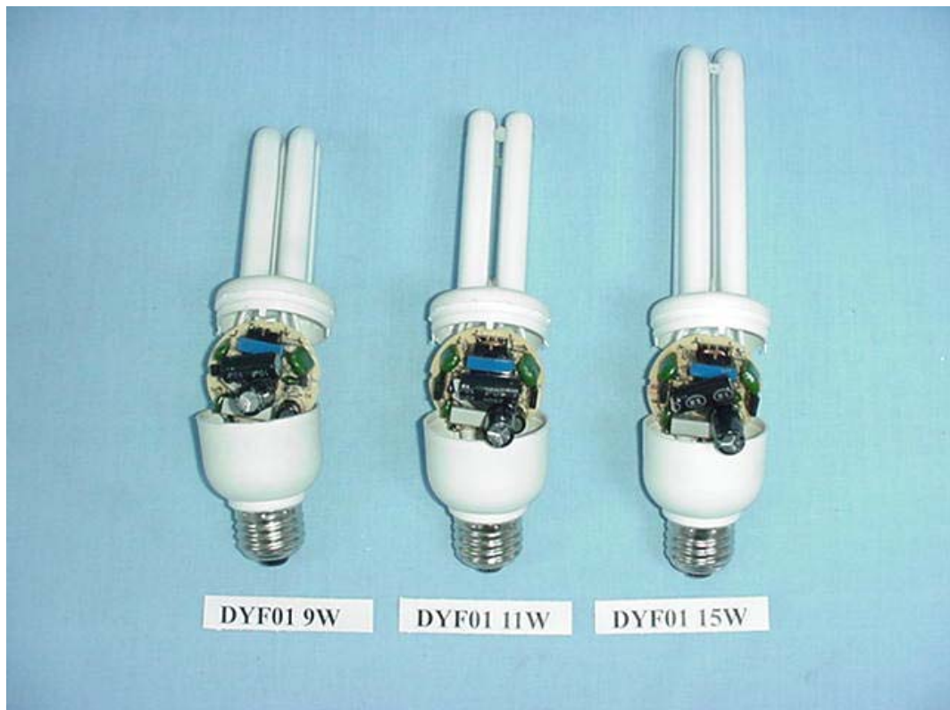
FIGURE 4 ENERGY SAVING LAMP (M/N: DYF01 9W 11W 15W) COVER REMOVED
