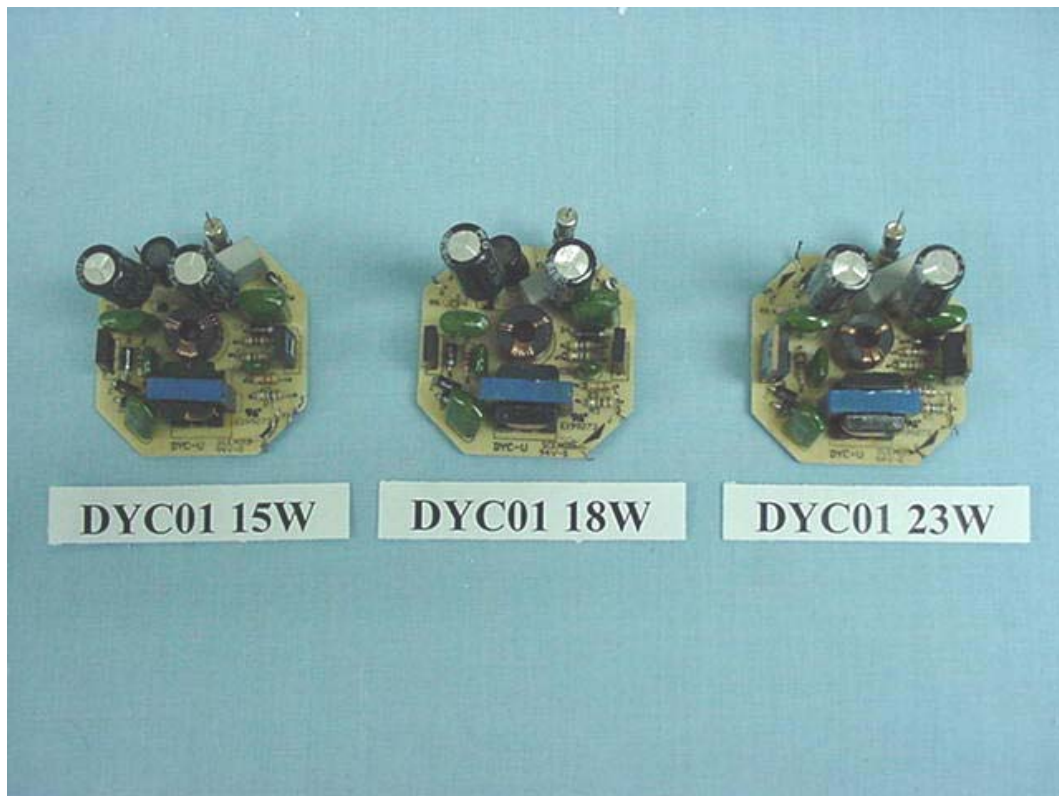
FIGURE 17 ENERGY SAVING LAMP (M/N: DYC01 15W 18W 23W) MAIN BOARD (COMPONENT SIDE)
