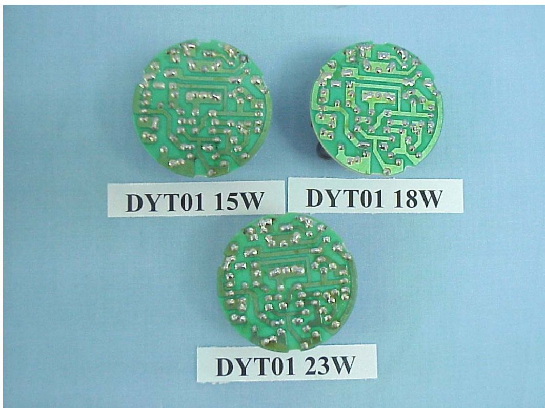
FIGURE 12 ENERGY SAVING LAMP (M/N: DYT01 15W 18W 23W) MAIN BOARD (SOLDERED SIDE)
