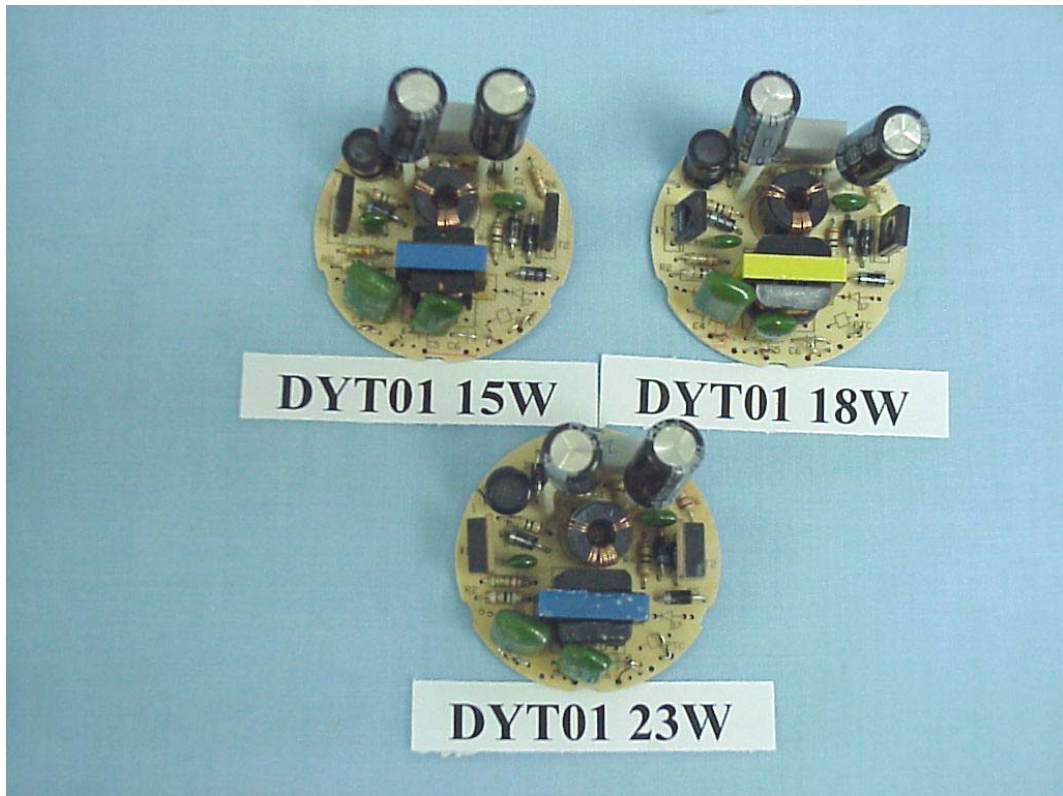
FIGURE 11 ENERGY SAVING LAMP (M/N: DYT01 15W 18W 23W) MAIN BOARD (COMPONENT SIDE)
