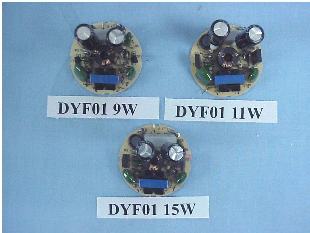
FIGURE 5 ENERGY SAVING LAMP (M/N: DYF01 9W 11W 15W) MAIN BOARD (COMPONENT SIDE)
