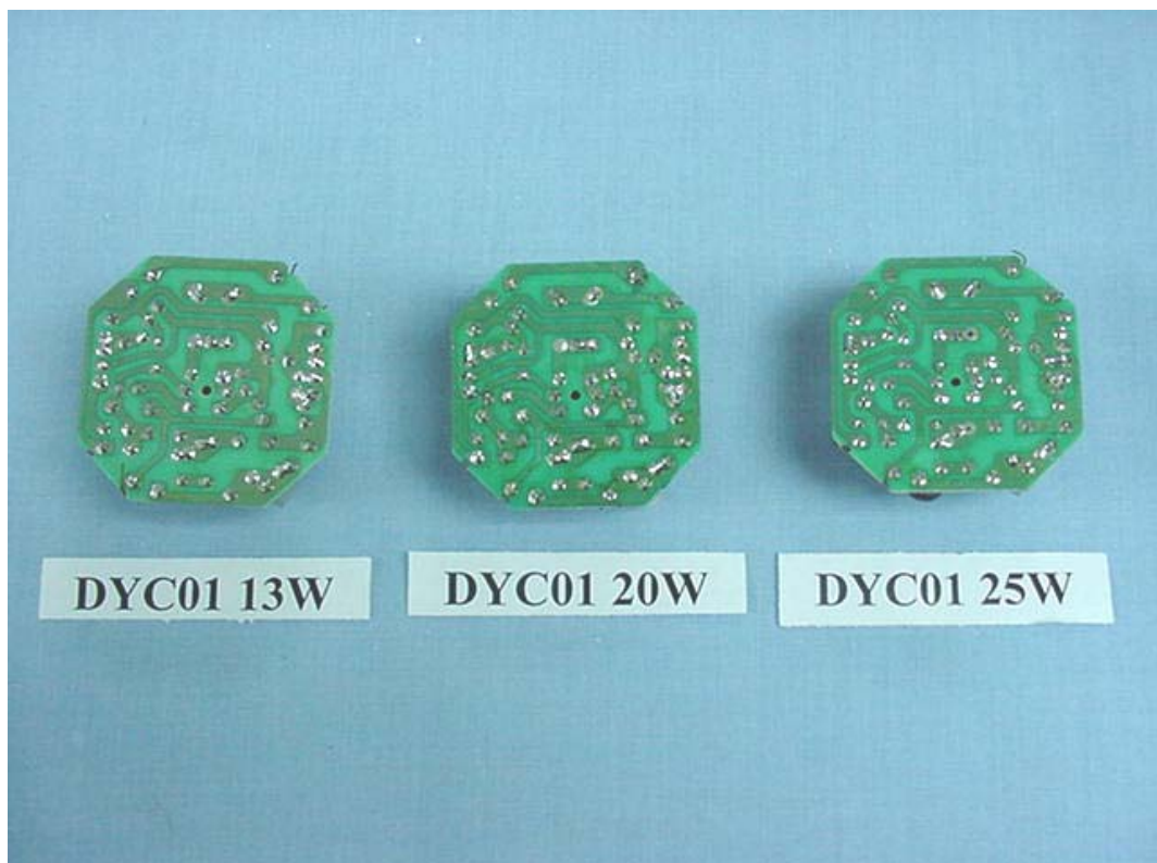
FIGURE 15 ENERGY SAVING LAMP (M/N: DYC01 13W 20W 25W) MAIN BOARD (SOLDERED SIDE)
