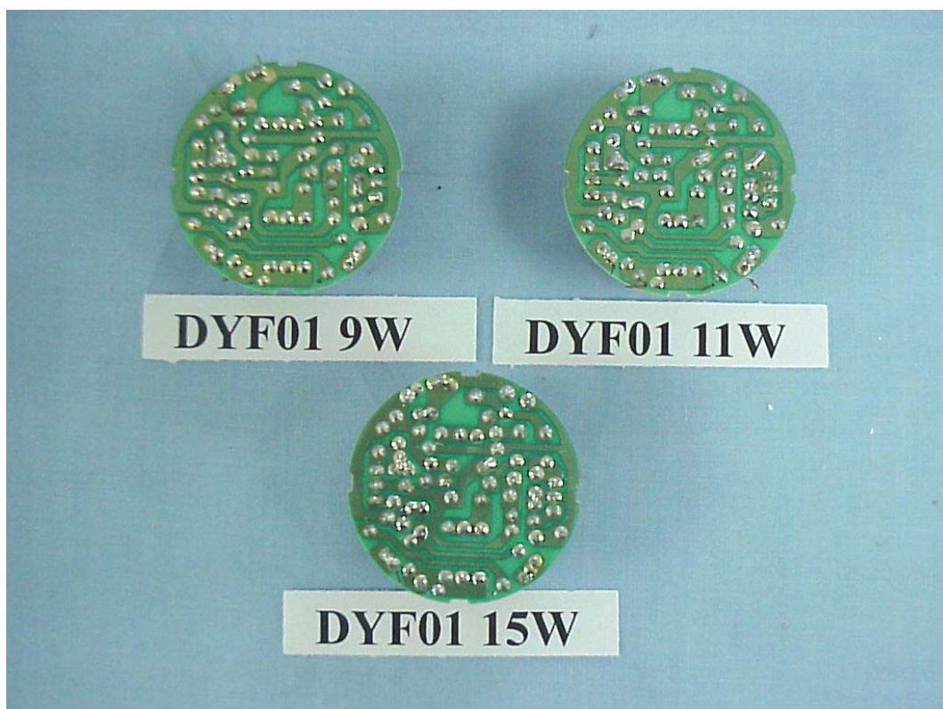
FIGURE 6 ENERGY SAVING LAMP (M/N: DYF01 9W 11W 15W) MAIN BOARD (SOLDERED SIDE)
