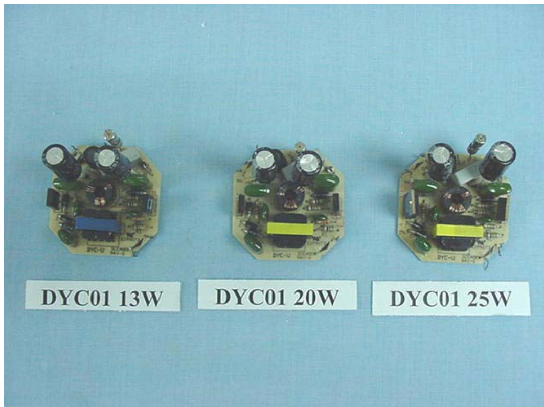
FIGURE 14 ENERGY SAVING LAMP (M/N: DYC01 13W 20W 25W) MAIN BOARD (COMPONENT SIDE)
