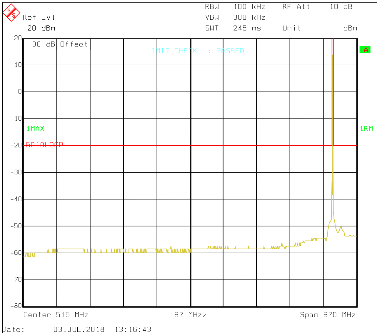
Plot 5-11: Conducted Antenna Spurious Emissions –929.0125 MHz; 30 MHz-1 GHz; 12.5 kHz BW; 20W
