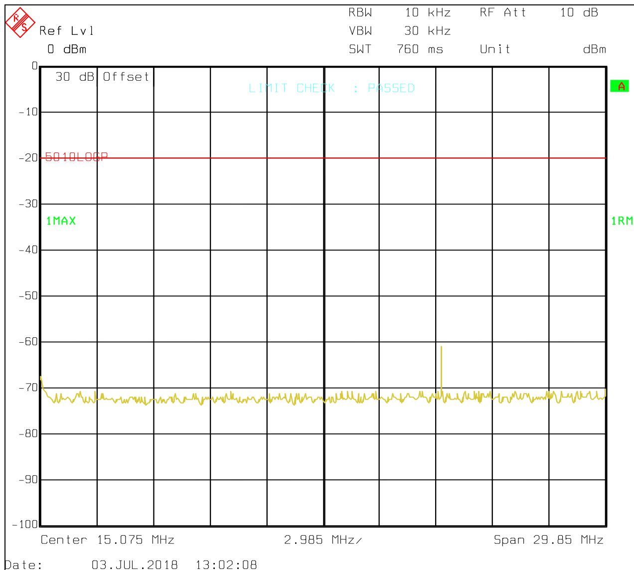
Plot 5-2: Conducted Antenna Spurious Emissions – 929.0125 MHz; 150 kHz-30 MHz; 12.5 kHz BW; 250W
