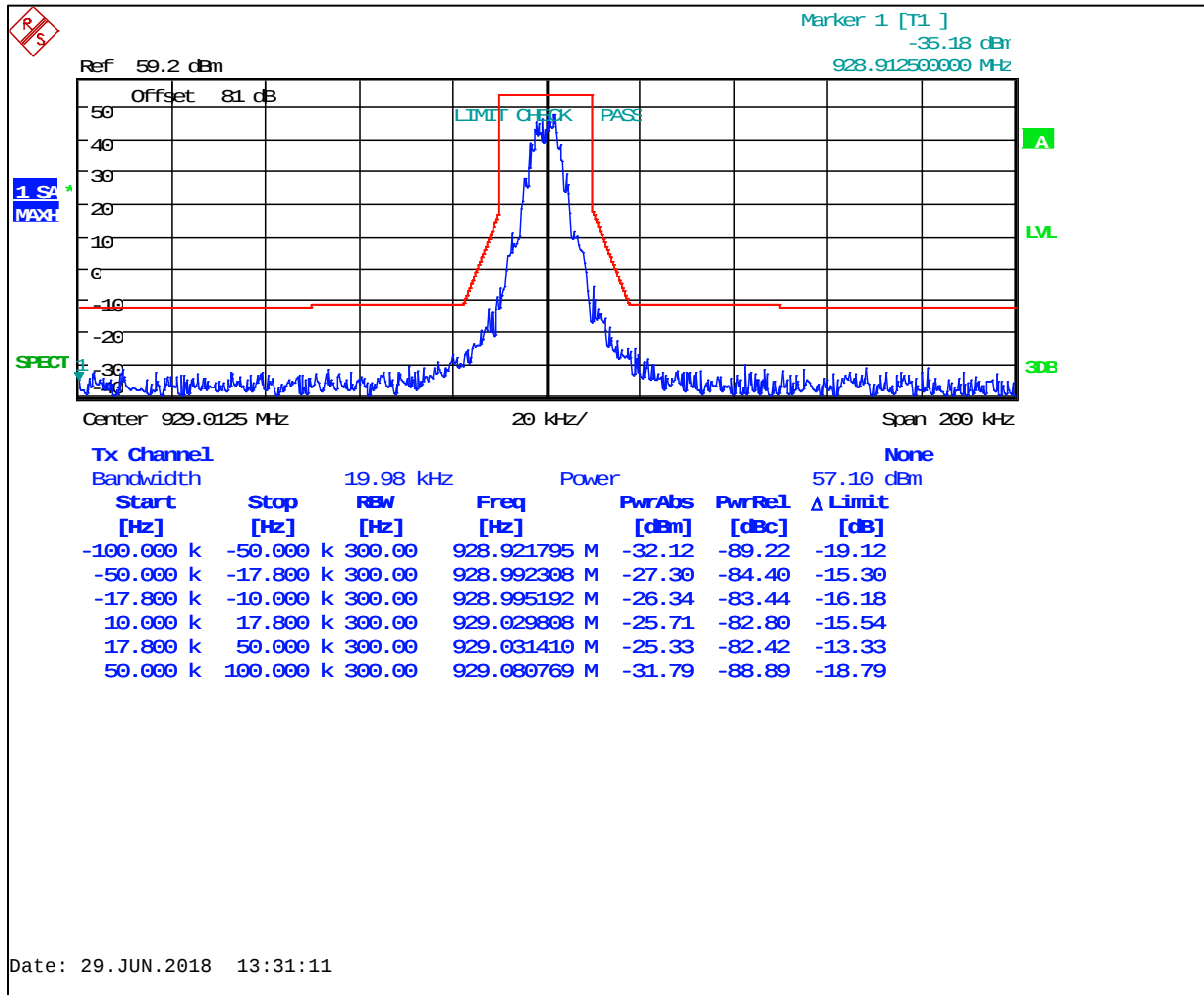
Plot 8-7: Emission Masks - 929.0125 MHz, 12.5 kHz Bandwidth, High Power; FLEX-4 6400 PRBS- Mask G
