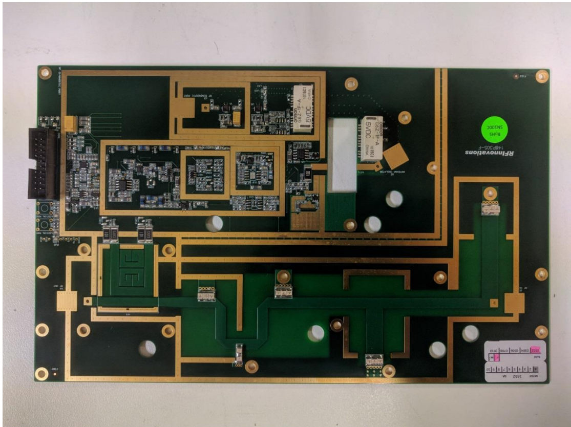
Isolator board top unshielded
