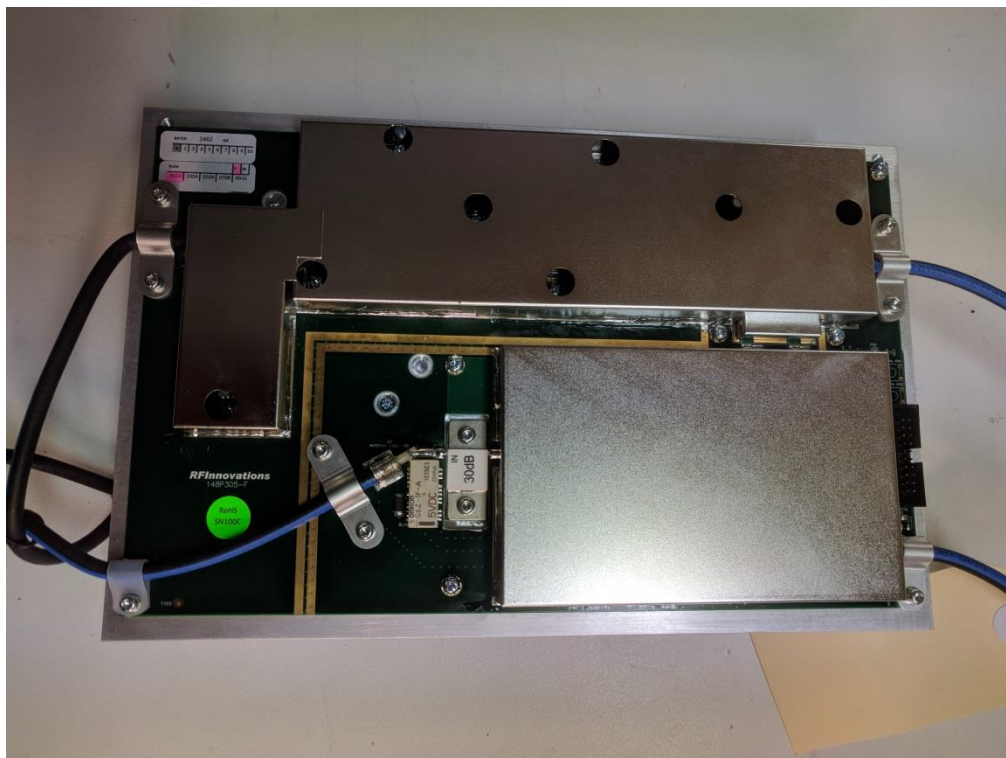
Isolator board top shielded
