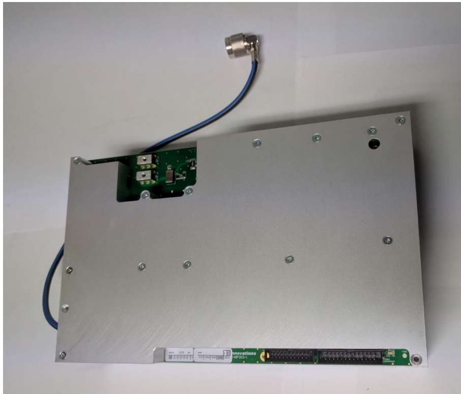
Power amplifier board top shielded
