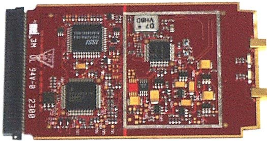
WLAN PCB Top view
