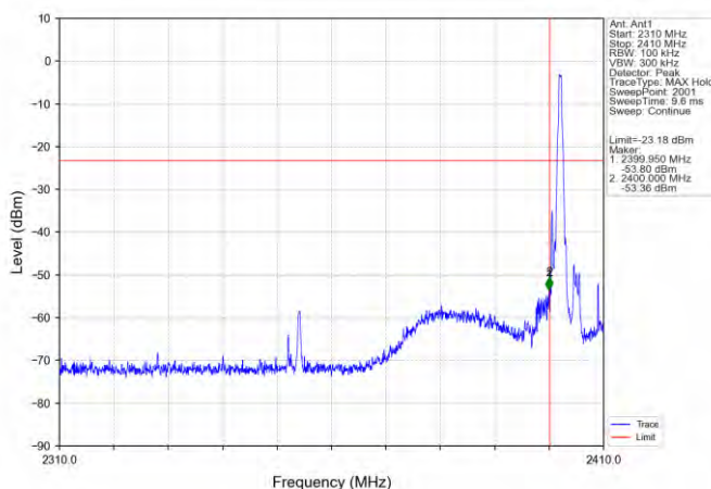
GFSK_DH5_LCH_2402MHz_Ant1_NTNV
