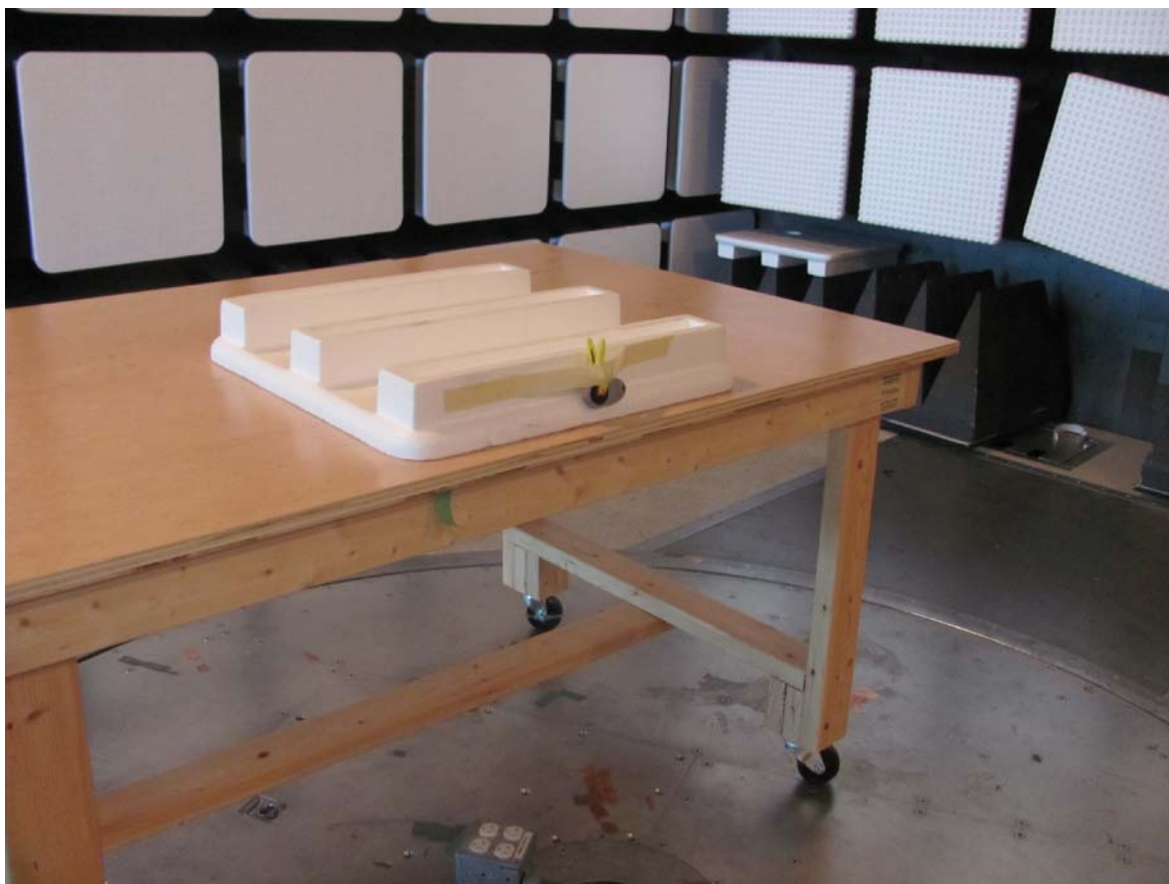
Illustration 9: Radiated emission setup – photo 4
