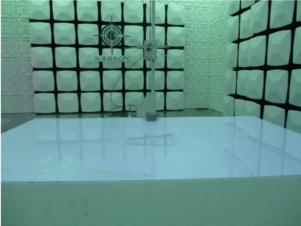
Setup Photo FCC ID: P59BST11 IC: 11242A-BST11
