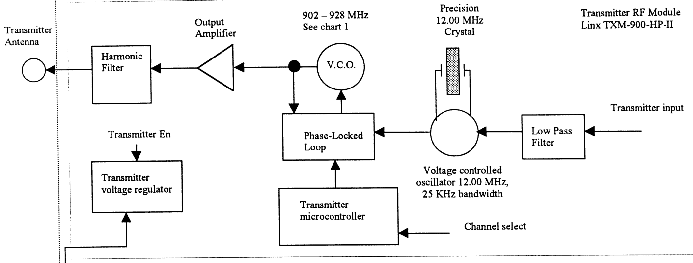
Transceiver Block Diagram
