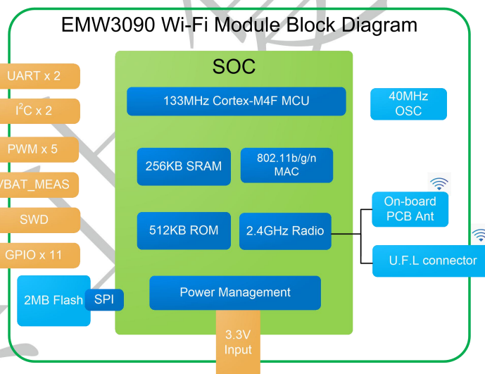
EMW3090 Hardware block
