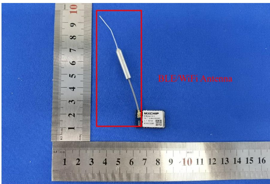
Photo 4: Antenna
