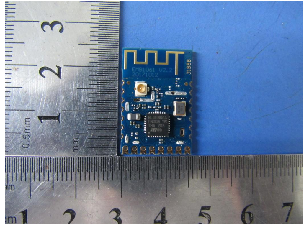
EUT(External Antenna) Uncover - Front View
