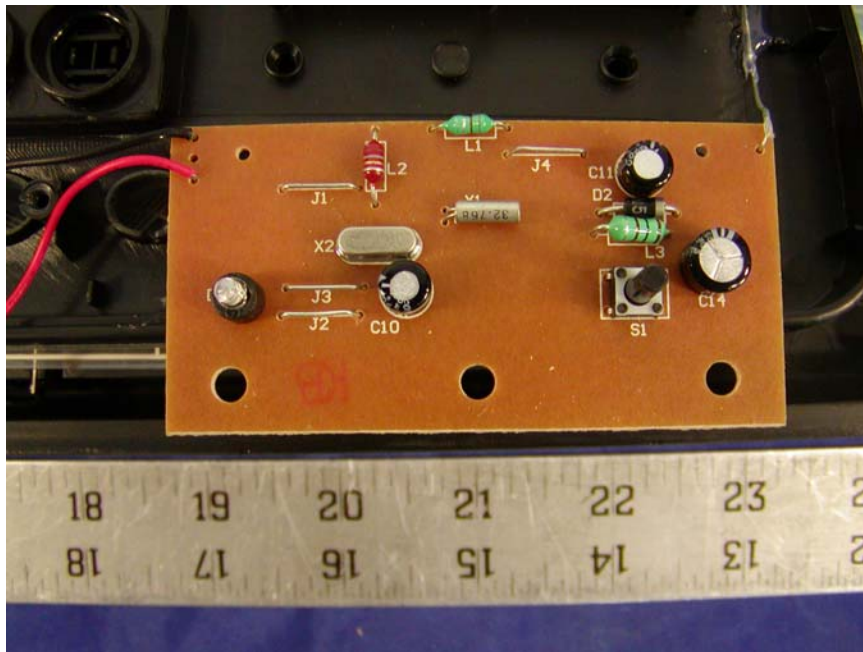
Transmitter Main Board – Component View
