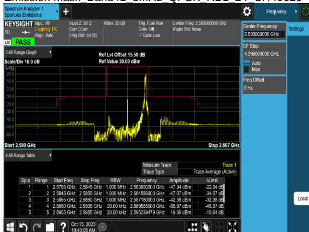
Emission Mask Band41 5MHz QPSK RB1 24 CH40620
