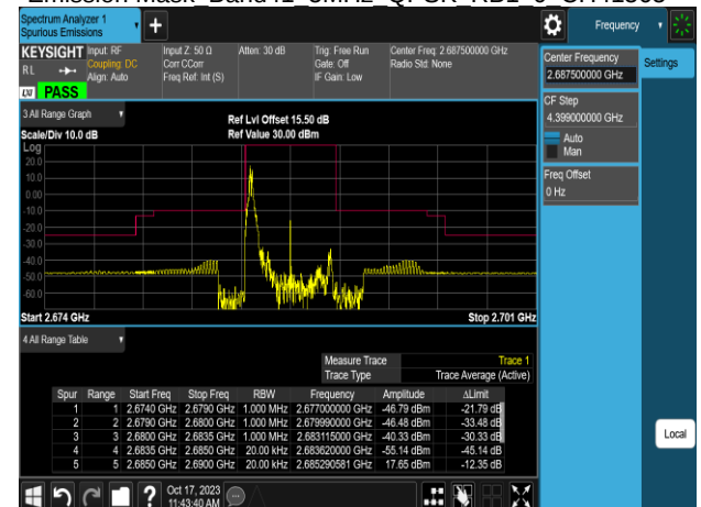
Emission Mask Band41 5MHz QPSK RB1 0 CH41565
