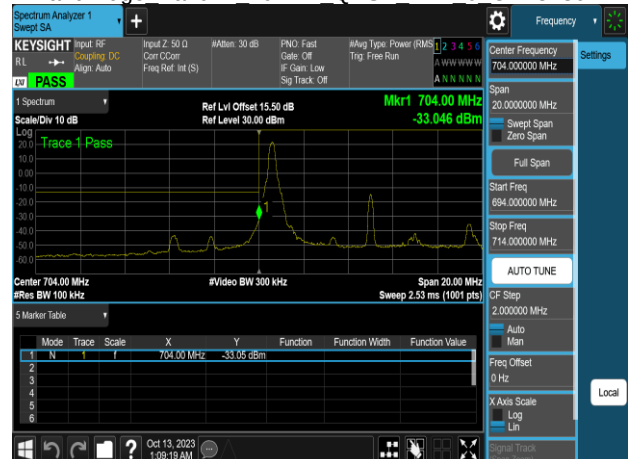
Band Edge Band17 10MHz QPSK RB1 0 CH23780
