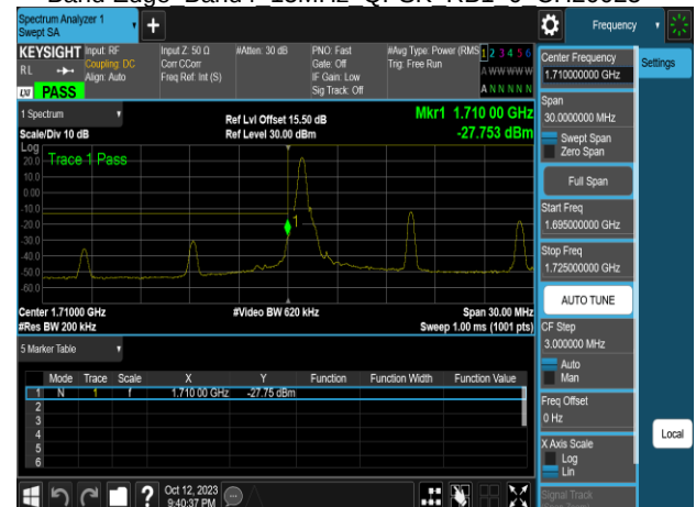
Band Edge Band4 15MHz QPSK RB1 74 CH20325
