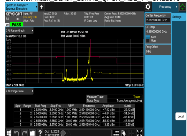
Emission Mask Band7 15MHz QPSK RB1 74 CH21375
