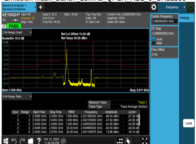
Emission Mask Band7 20MHz QPSK RB1 0 CH21350
