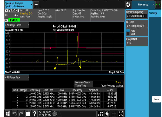
Emission Mask Band7 15MHz QPSK RB1 74 CH21100
