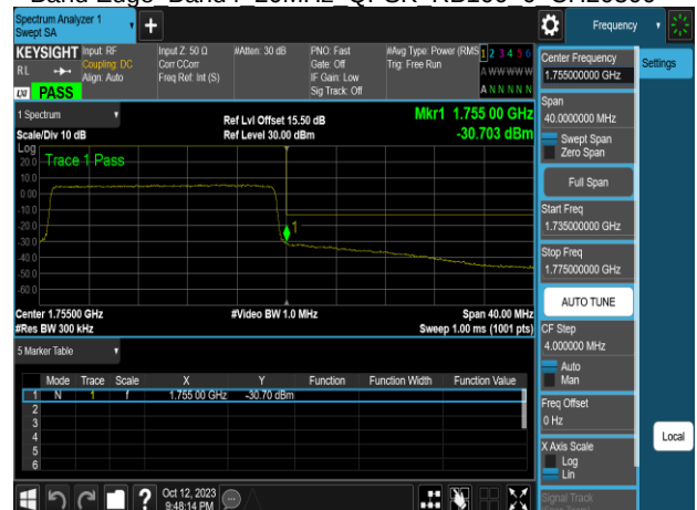
Band Edge Band4 20MHz QPSK RB100 0 CH20300
