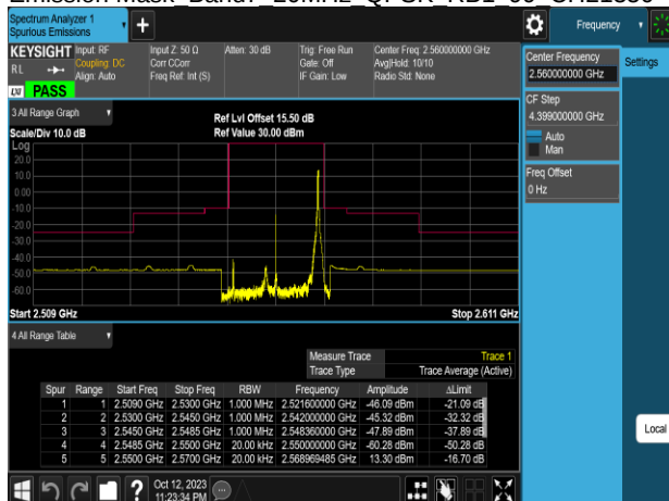
Emission Mask Band7 20MHz QPSK RB1 99 CH21350
