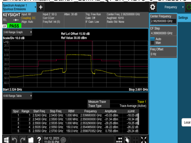
Emission Mask Band7 15MHz QPSK RB75 0 CH21375
