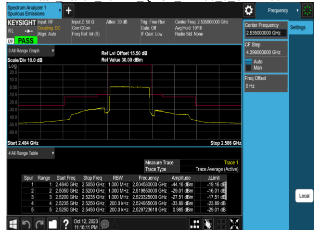
Emission Mask Band7 20MHz QPSK RB100 0 CH21350
