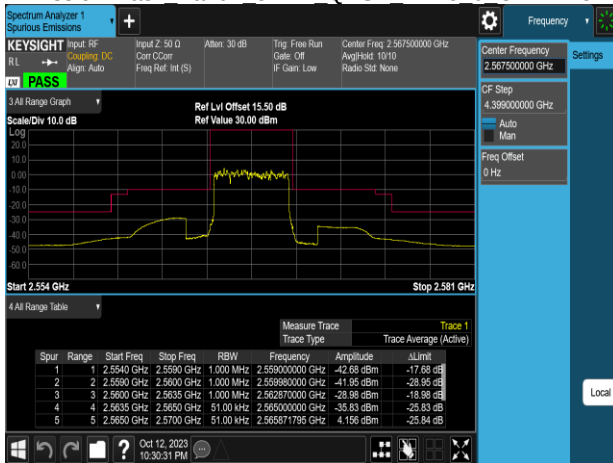
Emission Mask Band7 5MHz QPSK RB25 0 CH21425
