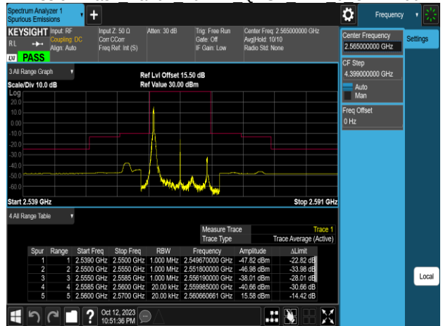
Emission Mask Band7 10MHz QPSK RB1 0 CH21400
