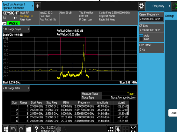
Emission Mask Band7 10MHz QPSK RB1 49 CH21400
