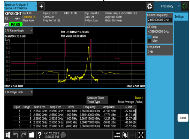
Emission Mask Band7 5MHz QPSK RB1 24 CH21425
