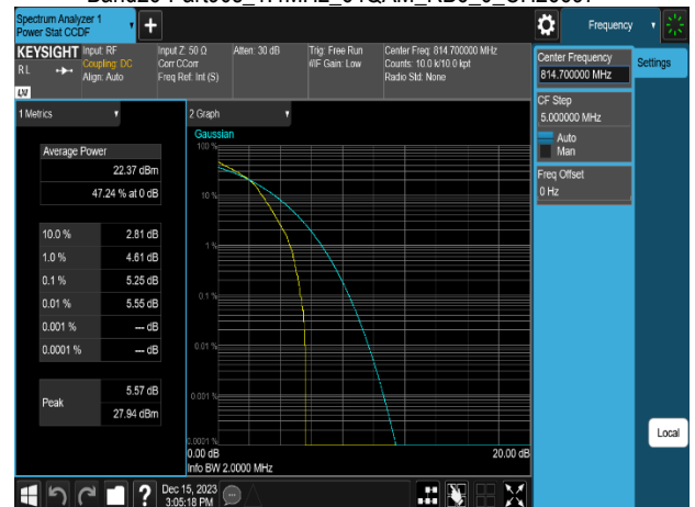
Band26-Part90s 1.4MHz 64QAM RB6 0 CH26697
