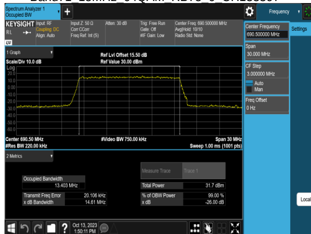
Band71 15MHz 64QAM RB75 0 CH133397
