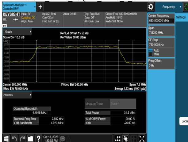
Band71 5MHz 16QAM RB25 0 CH133447
