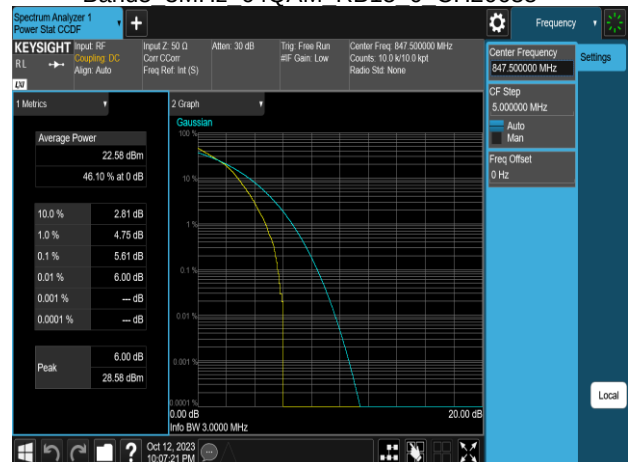
Band5 3MHz 64QAM RB15 0 CH20635
