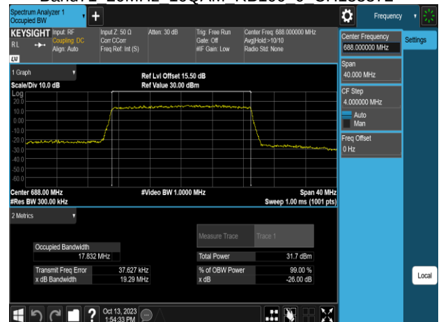
Band71 20MHz 16QAM RB100 0 CH133372
