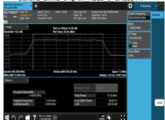
Band71 5MHz 64QAM RB25 0 CH133447
