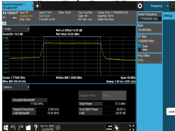
Band66 20MHz 64QAM RB100 0 CH132572
