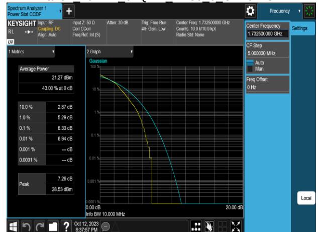
Band4 10MHz 64QAM RB50 0 CH20350
