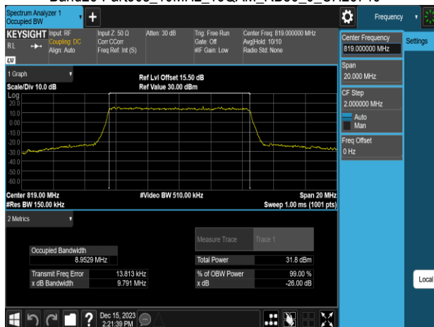
Band26-Part90s_10MHz_64QAM_RB50_0_CH26740
