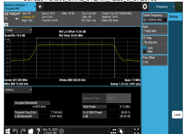
Band26-Part90s_5MHz_64QAM_RB25_0_CH26765
