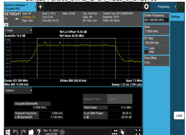
Band26-Part90s_5MHz_QPSK_RB25_0_CH26765
