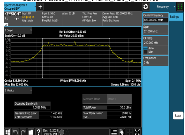
Band26-Part90s_1.4MHz_64QAM_RB6_0_CH26783
