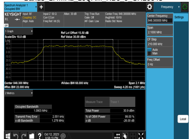
Band5 1.4MHz 16QAM RB6 0 CH20643
