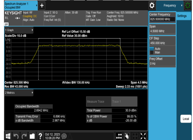
Band5 3MHz 64QAM RB15 0 CH20525
