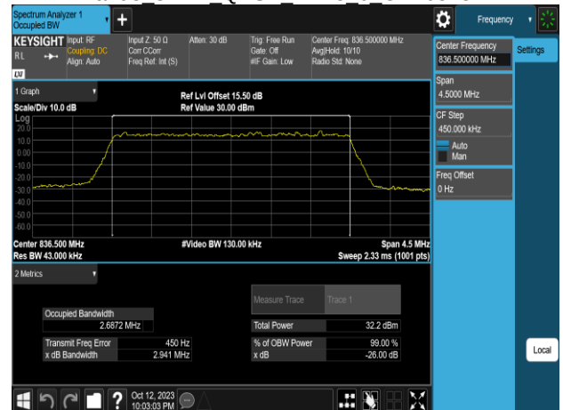
Band5 3MHz QPSK RB15 0 CH20635
