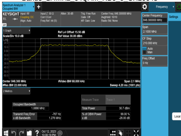
Band5 1.4MHz 64QAM RB6 0 CH20643
