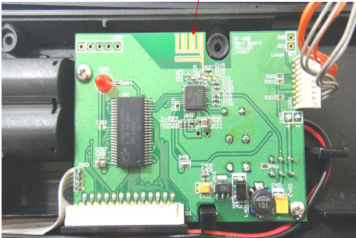
Printed Antenna
