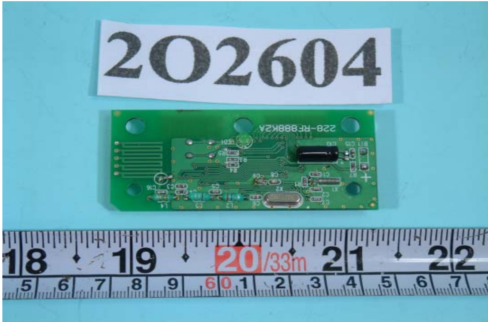
Rear side of Main Board
