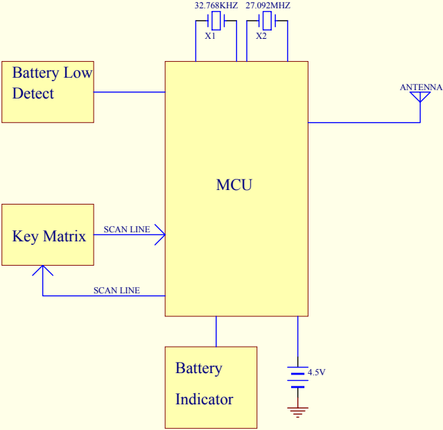
RF-888 BLOCK DIAGRAM
