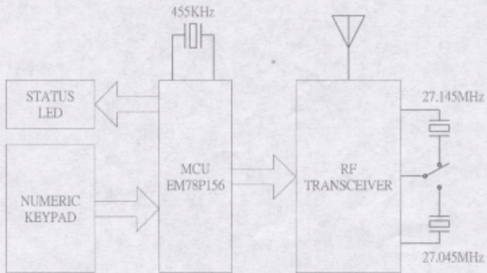
RF-525TX BLOCK DIAGRAM
