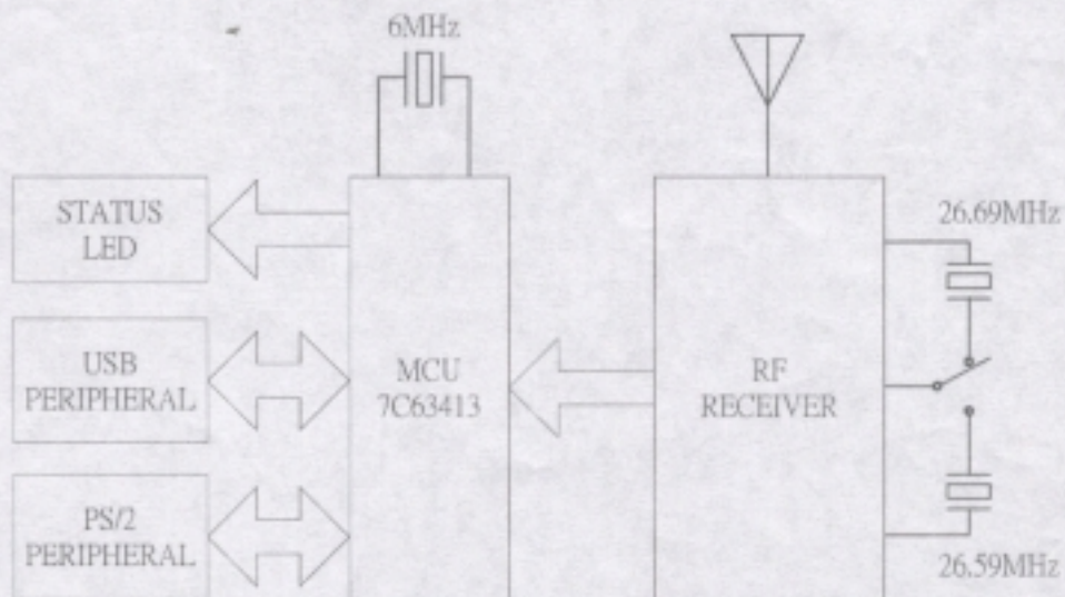
RF-525RX BLOCK DIAGRAM
