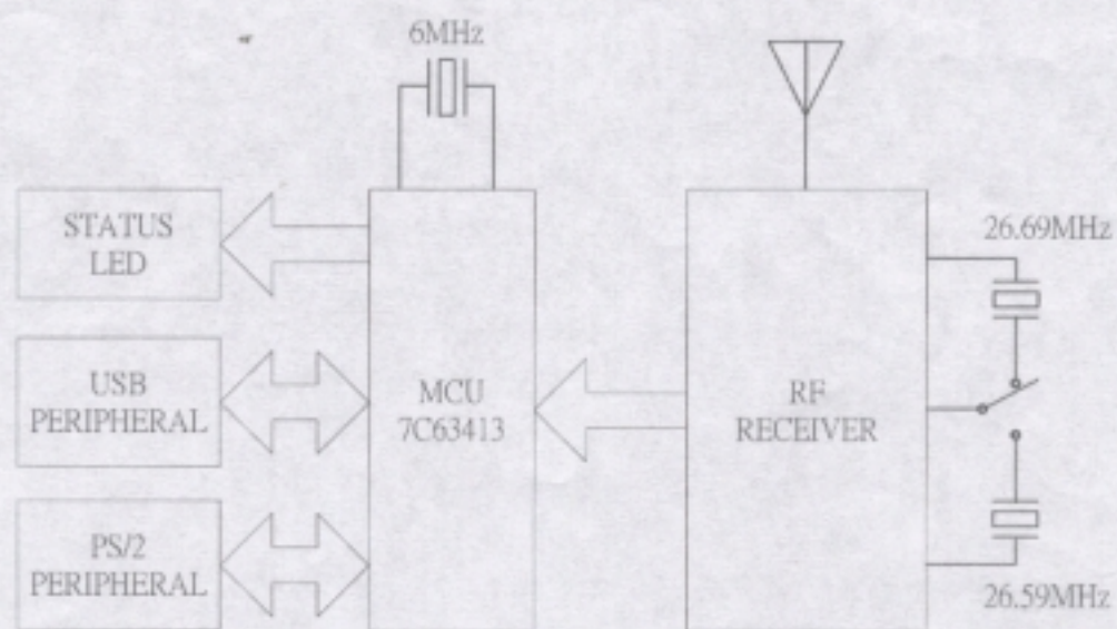
RF-540RX BLOCK DIAGRAM
