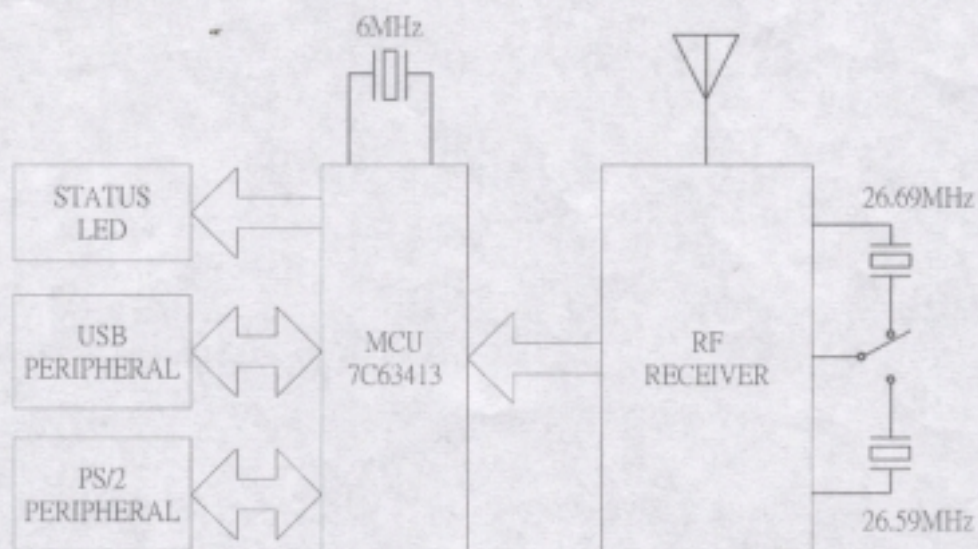
RF-530RX BLOCK DIAGRAM
