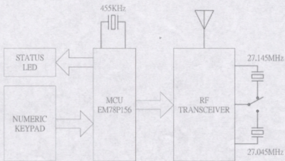
RF-530TX BLOCK DIAGRAM
