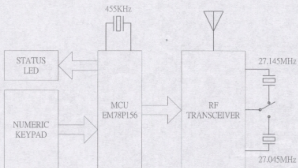
RF-540TX BLOCK DIAGRAM
