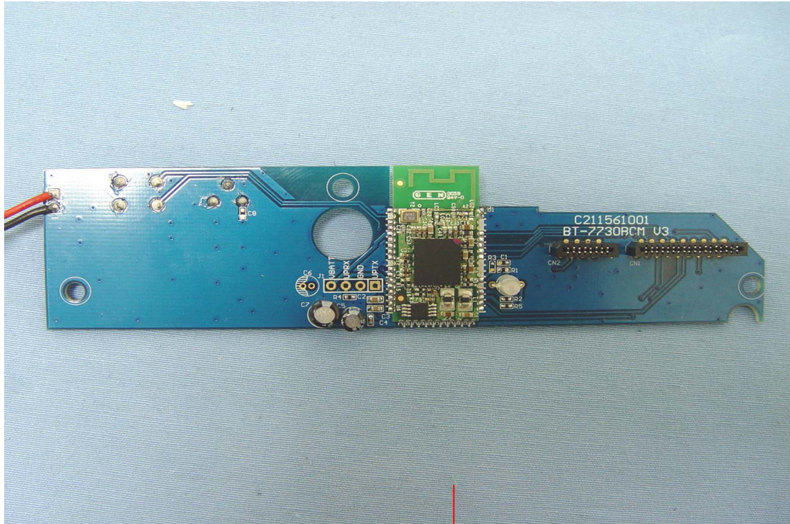
PCB Antenna
