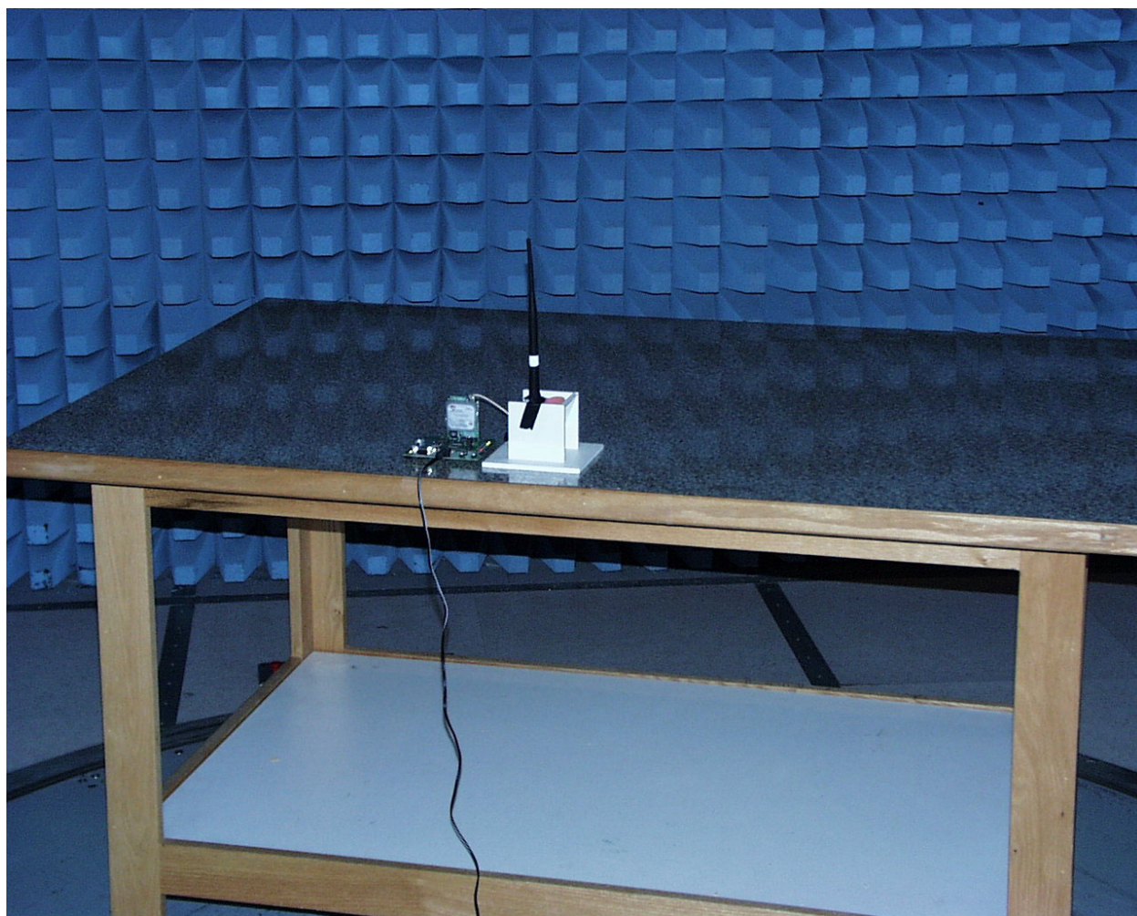
Front View of the Radiated Test Setup
