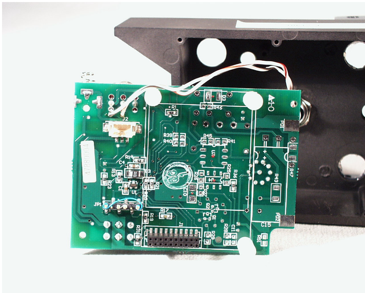
Bottom view of the RFD PCB
