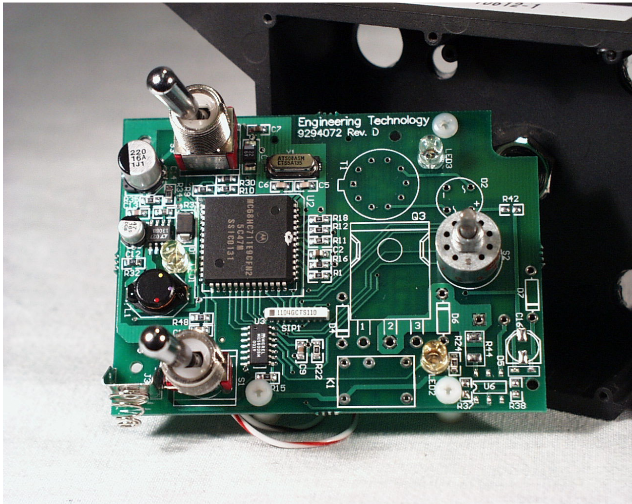
Top view of the RFD PCB
