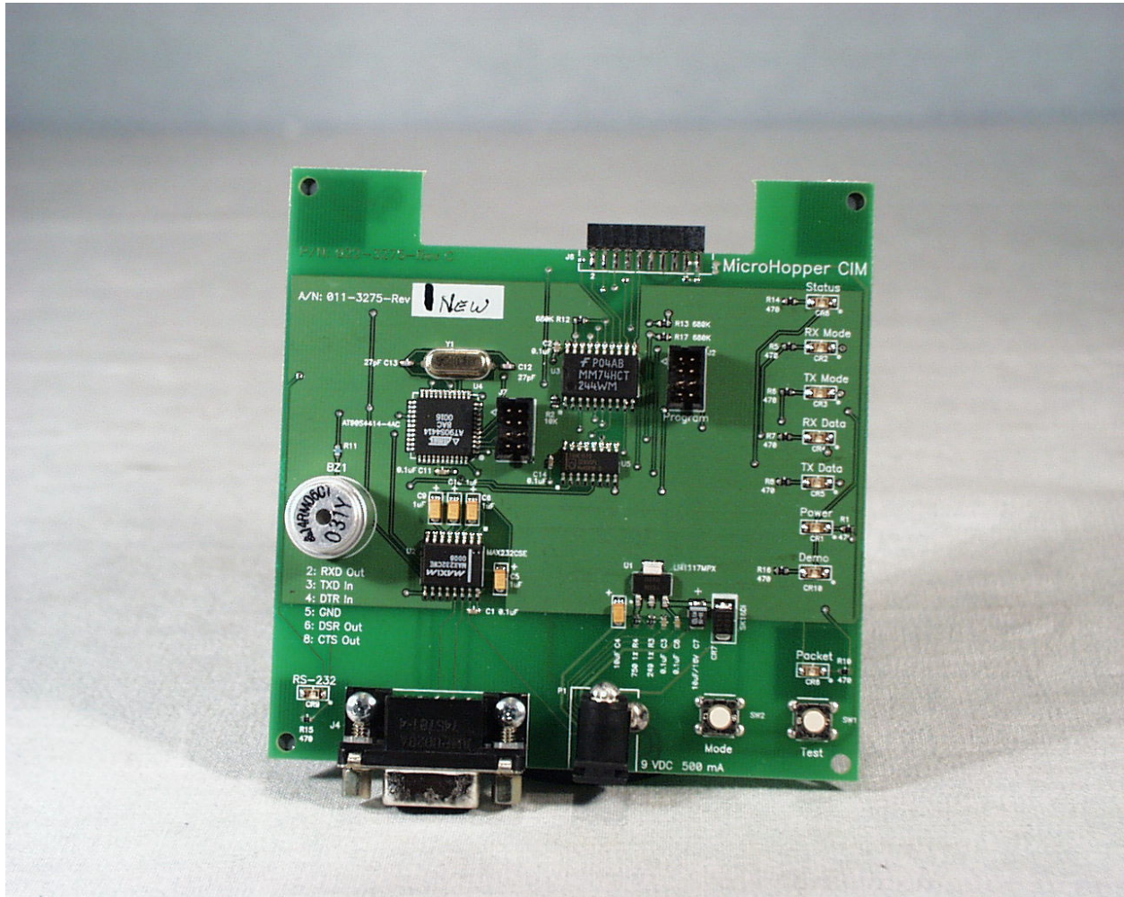
Top view of the RF test board
