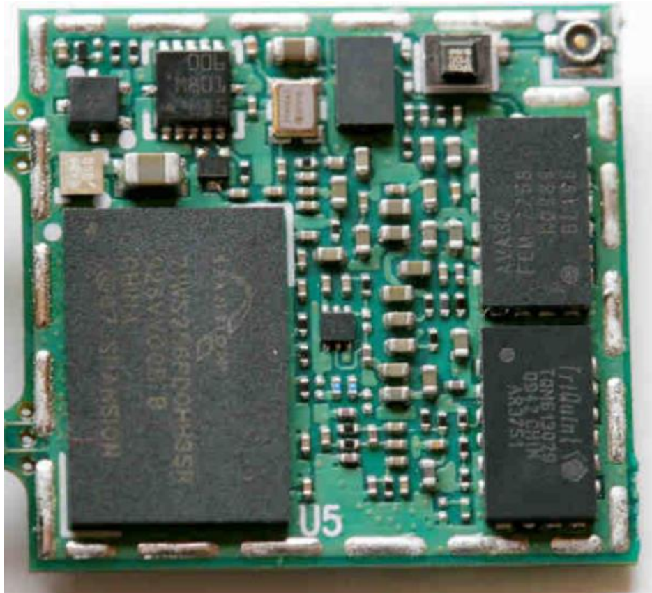
Module internal (side 1)
