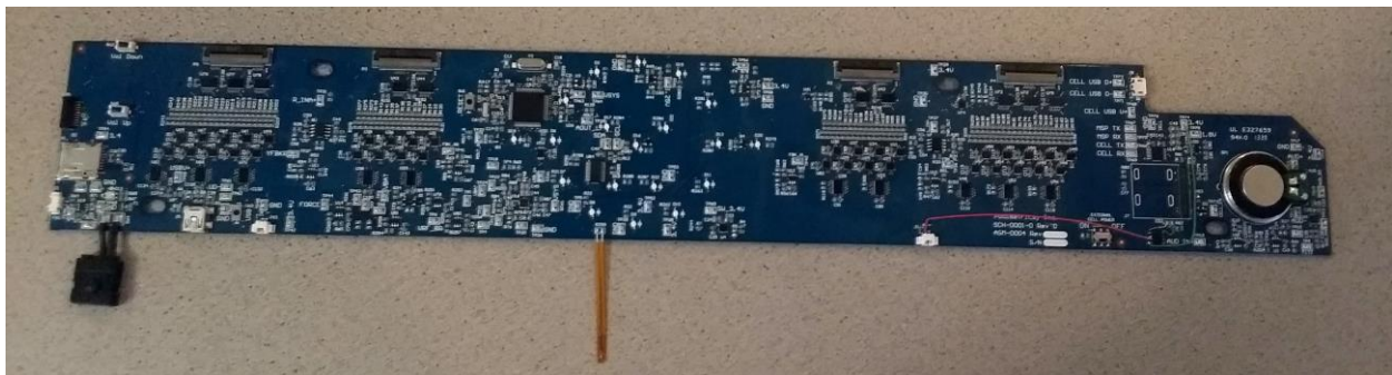
Top view of circuit board (with no cellular module populated)
