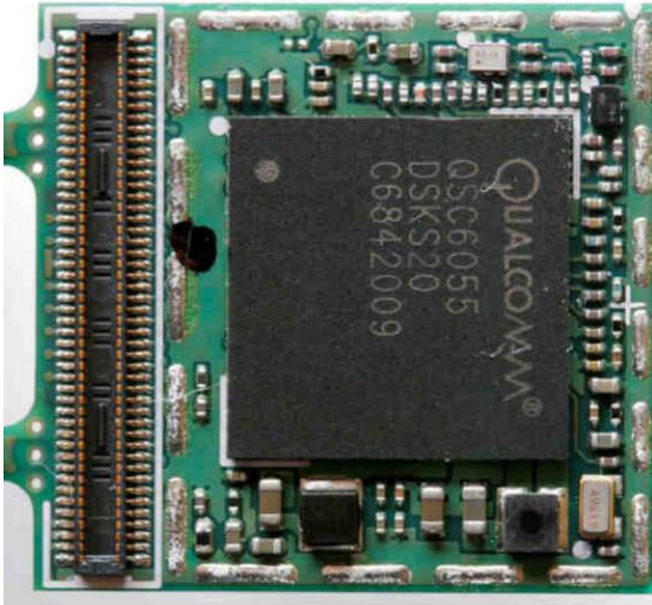
Module internal (side 2)
