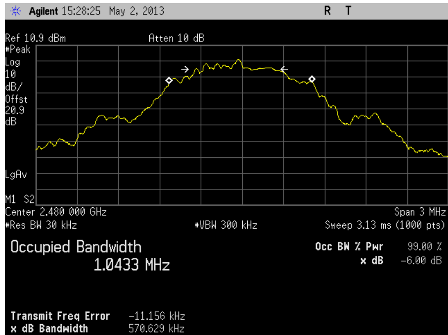
Bluetooth LE High Channel
