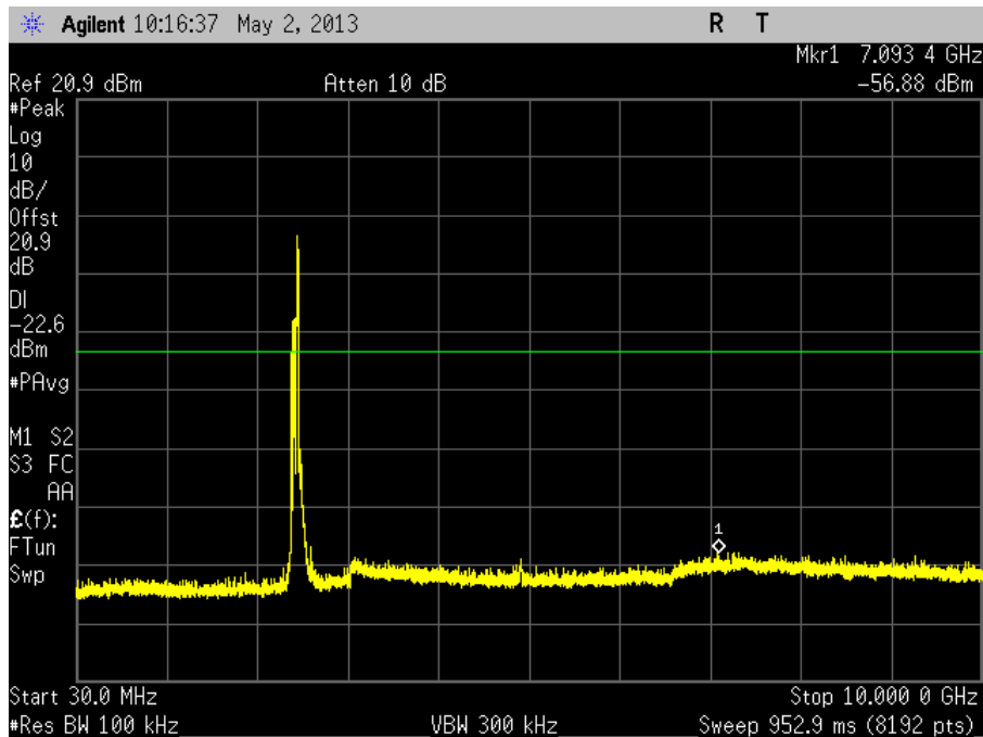
802.11n High Channel (30MHz to 10GHz)
