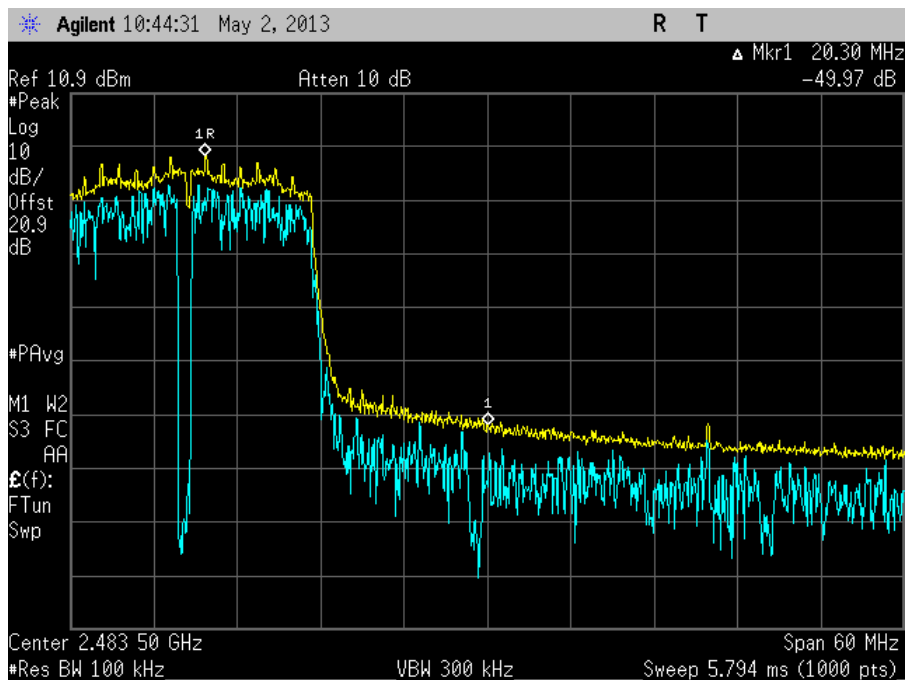
802.11n High Channel (2462 MHz)
