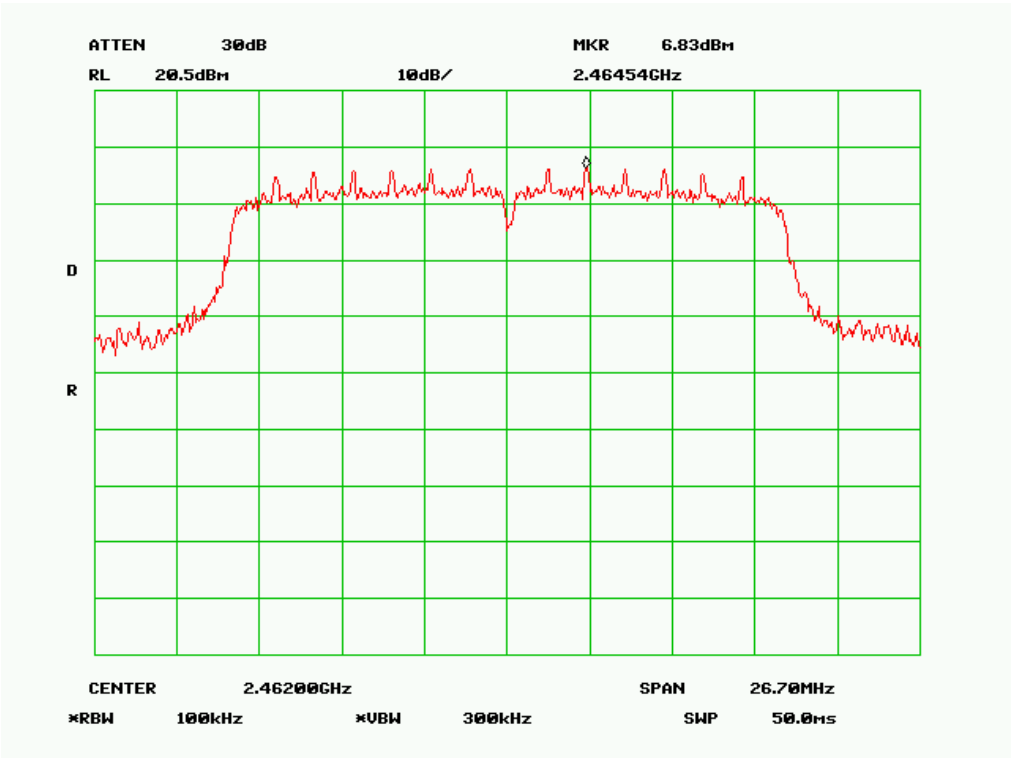
Power Spectral Density, 802.11n High Channel
