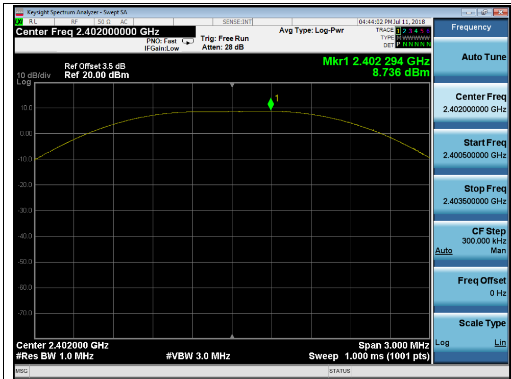
(Channel 0, 2402MHz)
