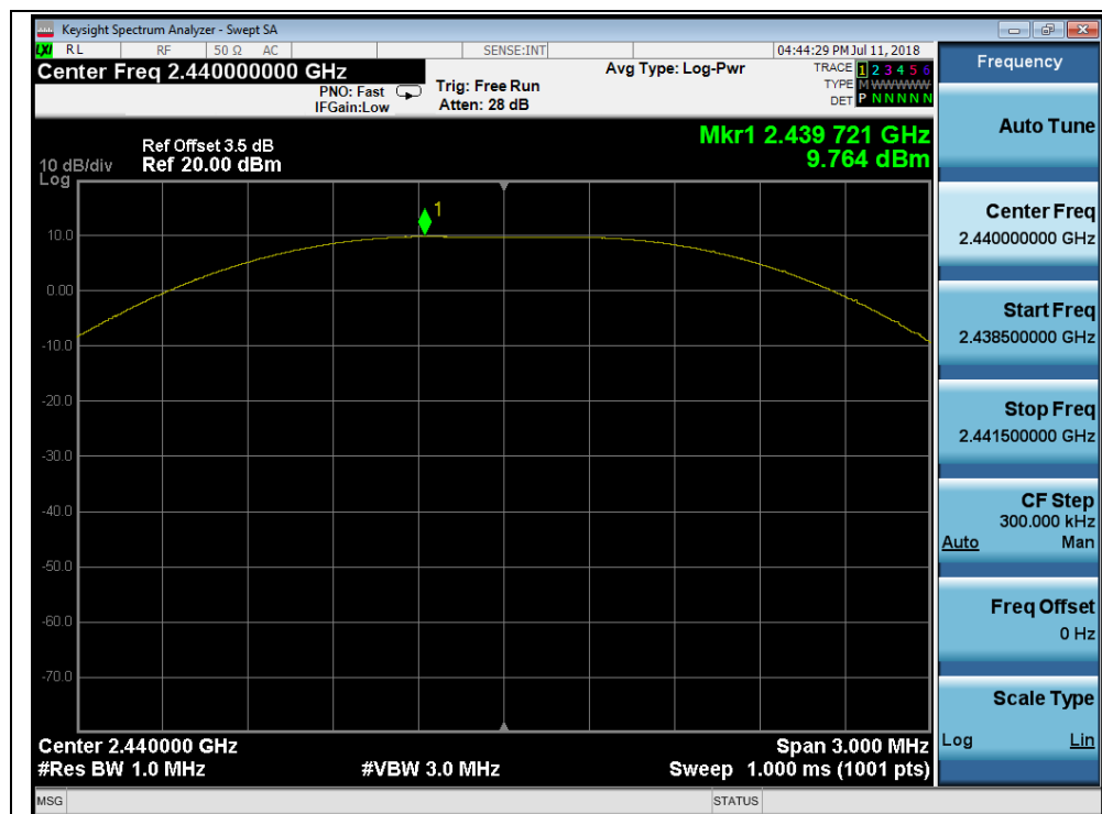
(Channel 19, 2440MHz)
